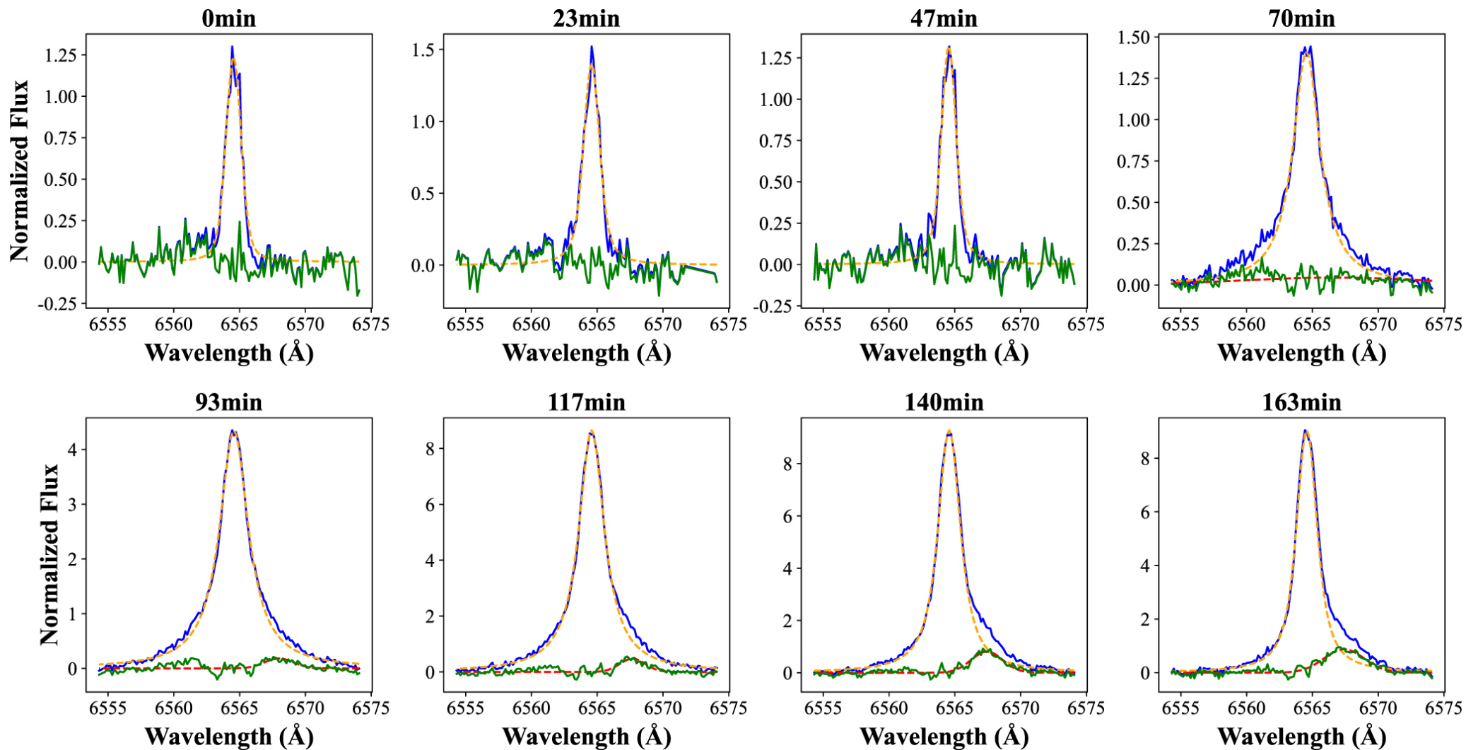
Figure 3. from Yuchuan Wu et al 2022 Astrophys. J. 928 doi:10.3847/1538-4357/ac5897 https://dx.doi.org/10.3847/1538-4357/ac5897 © 2022. The Author(s). Published by the American Astronomical Society.
