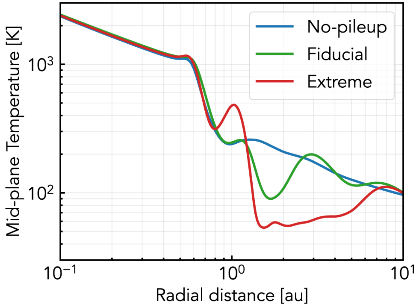
Figure 7. from Probing the Inner Edge of Dead Zones in Protoplanetary Disks with ALMA and Next Generation Very Large Array null 2022 APJ 928 110 doi:10.3847/1538-4357/ac56d8 https://dx.doi.org/10.3847/1538-4357/ac56d8 © 2022. The Author(s). Published by the American Astronomical Society.
