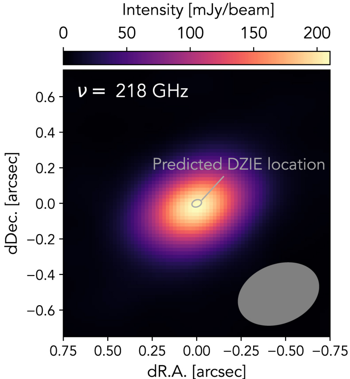
Figure 6. from Probing the Inner Edge of Dead Zones in Protoplanetary Disks with ALMA and Next Generation Very Large Array null 2022 APJ 928 110 doi:10.3847/1538-4357/ac56d8 https://dx.doi.org/10.3847/1538-4357/ac56d8 © 2022. The Author(s). Published by the American Astronomical Society.
