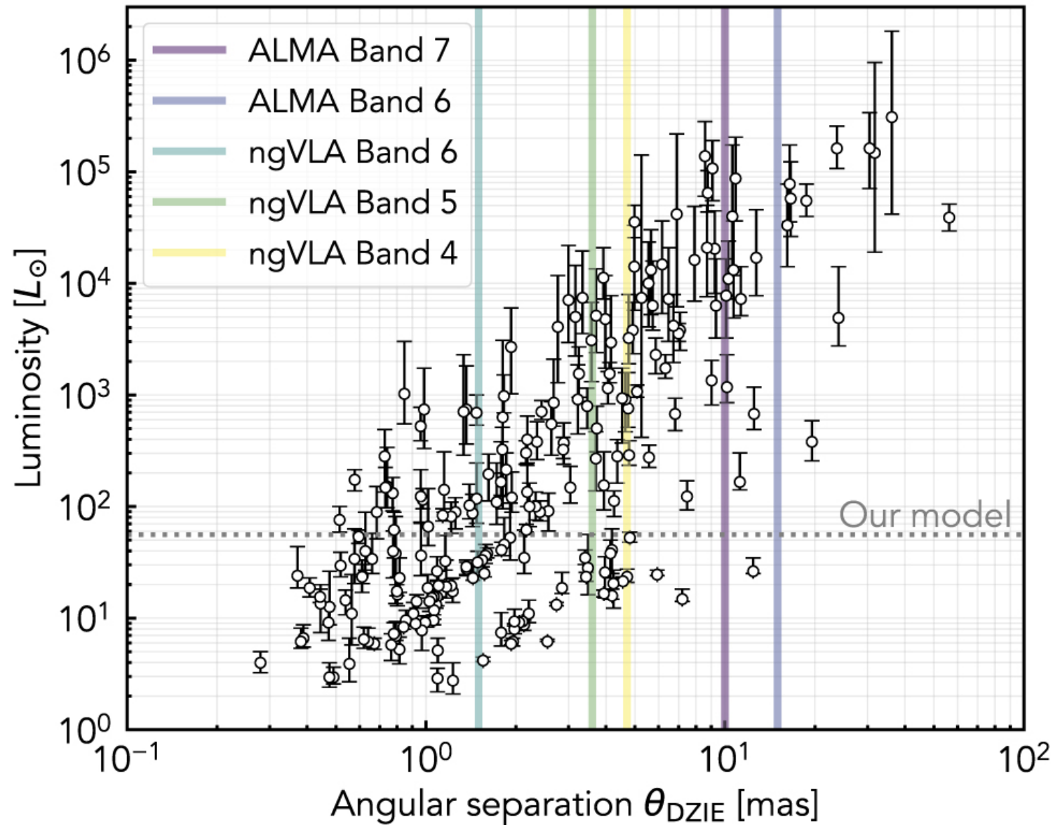
Figure 5. from Probing the Inner Edge of Dead Zones in Protoplanetary Disks with ALMA and Next Generation Very Large Array null 2022 APJ 928 110 doi:10.3847/1538-4357/ac56d8 https://dx.doi.org/10.3847/1538-4357/ac56d8 © 2022. The Author(s). Published by the American Astronomical Society.
