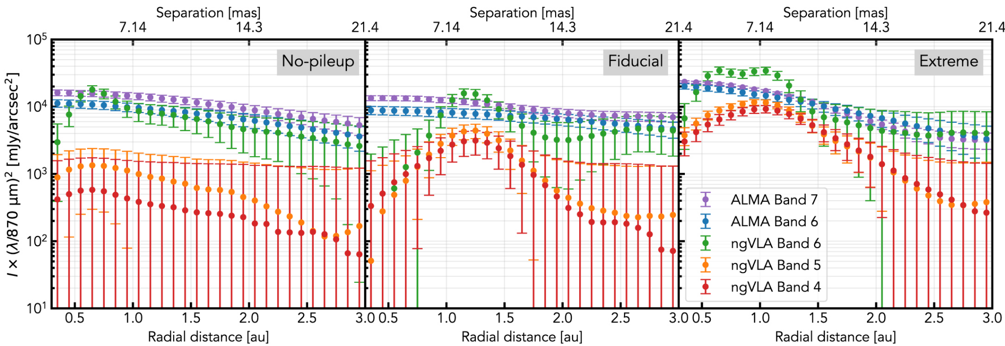
Figure 4. from Probing the Inner Edge of Dead Zones in Protoplanetary Disks with ALMA and Next Generation Very Large Array null 2022 APJ 928 110 doi:10.3847/1538-4357/ac56d8 https://dx.doi.org/10.3847/1538-4357/ac56d8 © 2022. The Author(s). Published by the American Astronomical Society.
