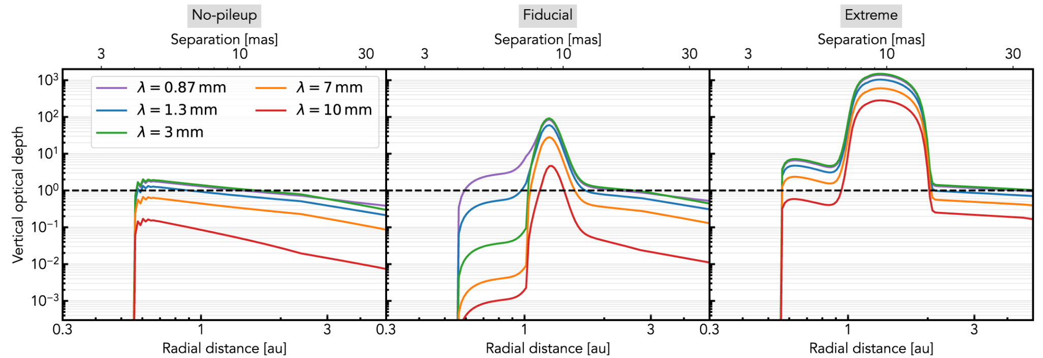
Figure 2. from Probing the Inner Edge of Dead Zones in Protoplanetary Disks with ALMA and Next Generation Very Large Array null 2022 APJ 928 110 doi:10.3847/1538-4357/ac56d8 https://dx.doi.org/10.3847/1538-4357/ac56d8 © 2022. The Author(s). Published by the American Astronomical Society.
