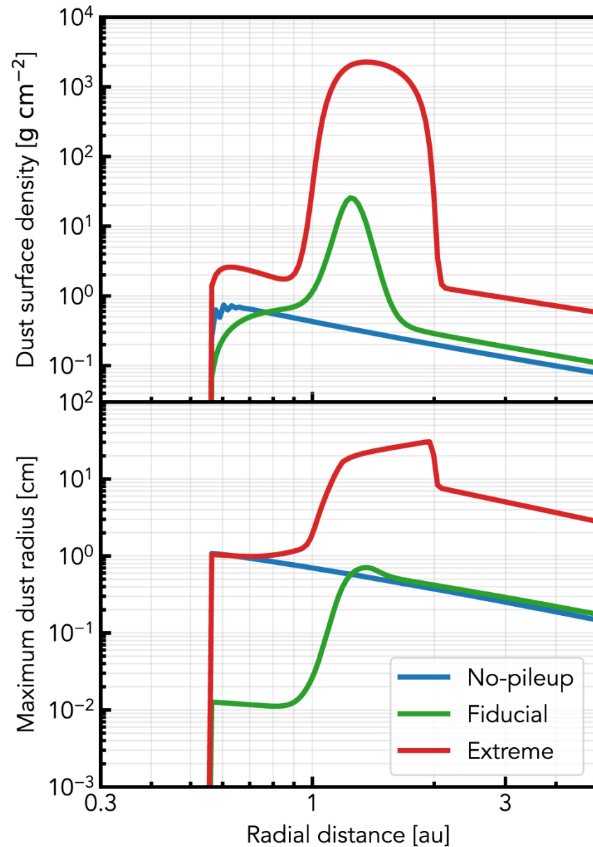
Figure 1. from Probing the Inner Edge of Dead Zones in Protoplanetary Disks with ALMA and Next Generation Very Large Array null 2022 APJ 928 110 doi:10.3847/1538-4357/ac56d8 https://dx.doi.org/10.3847/1538-4357/ac56d8 © 2022. The Author(s). Published by the American Astronomical Society.
