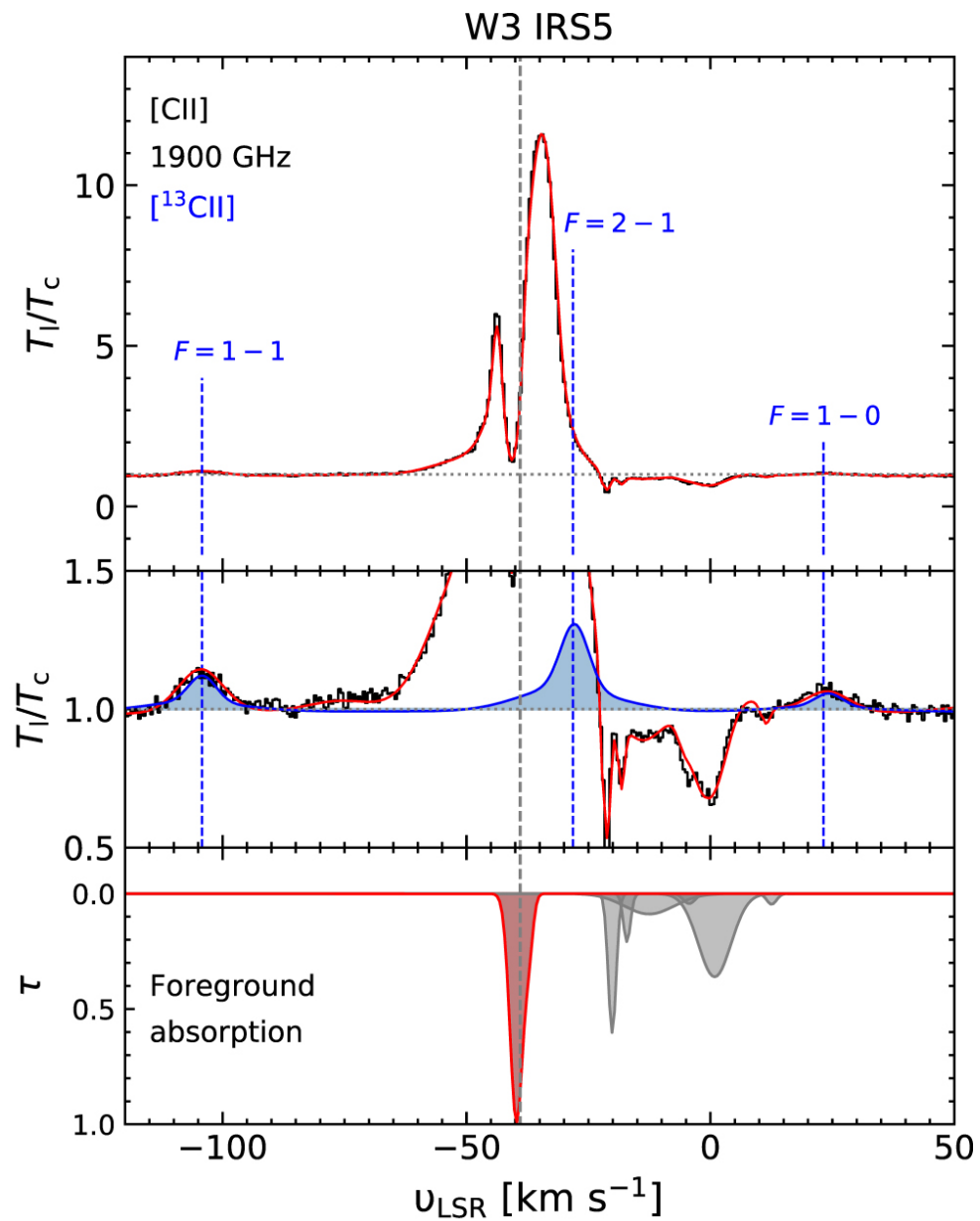
Figure 16. from A. M. Jacob et al 2022 Astrophys. J. 930 doi:10.3847/1538-4357/ac5409 https://dx.doi.org/10.3847/1538-4357/ac5409 © 2022. The Author(s). Published by the American Astronomical Society.
