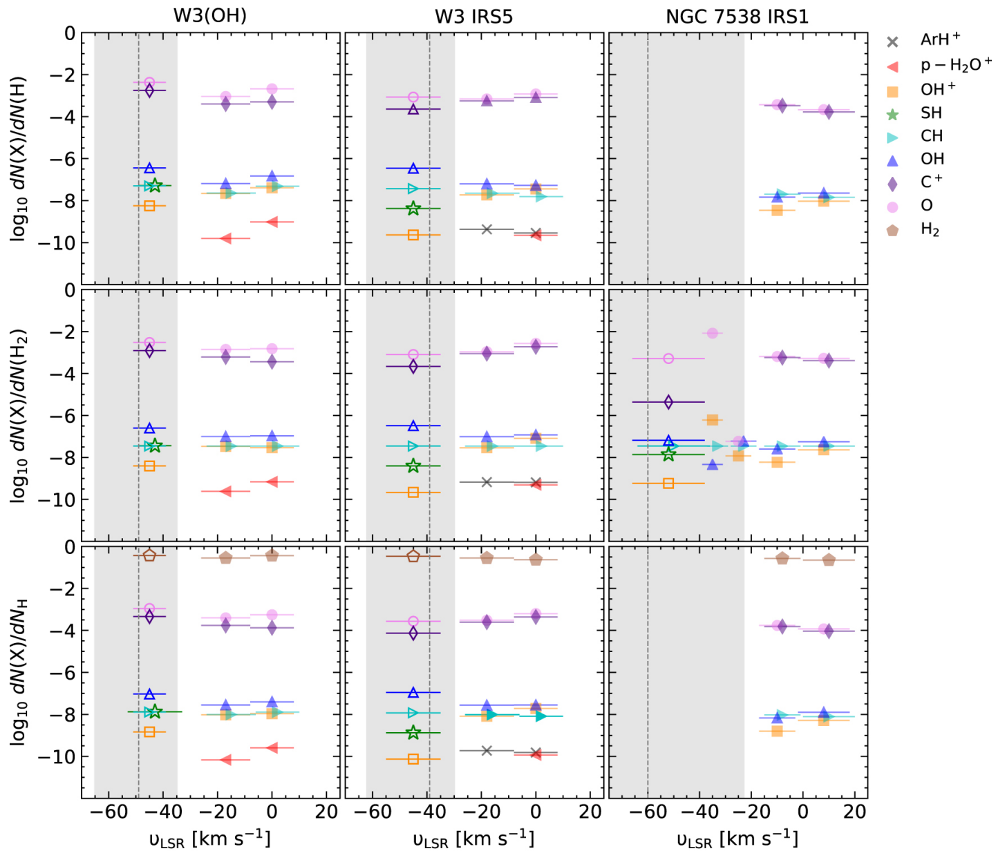
Figure 14. from A. M. Jacob et al 2022 Astrophys. J. 930 doi:10.3847/1538-4357/ac5409 https://dx.doi.org/10.3847/1538-4357/ac5409 © 2022. The Author(s). Published by the American Astronomical Society.
