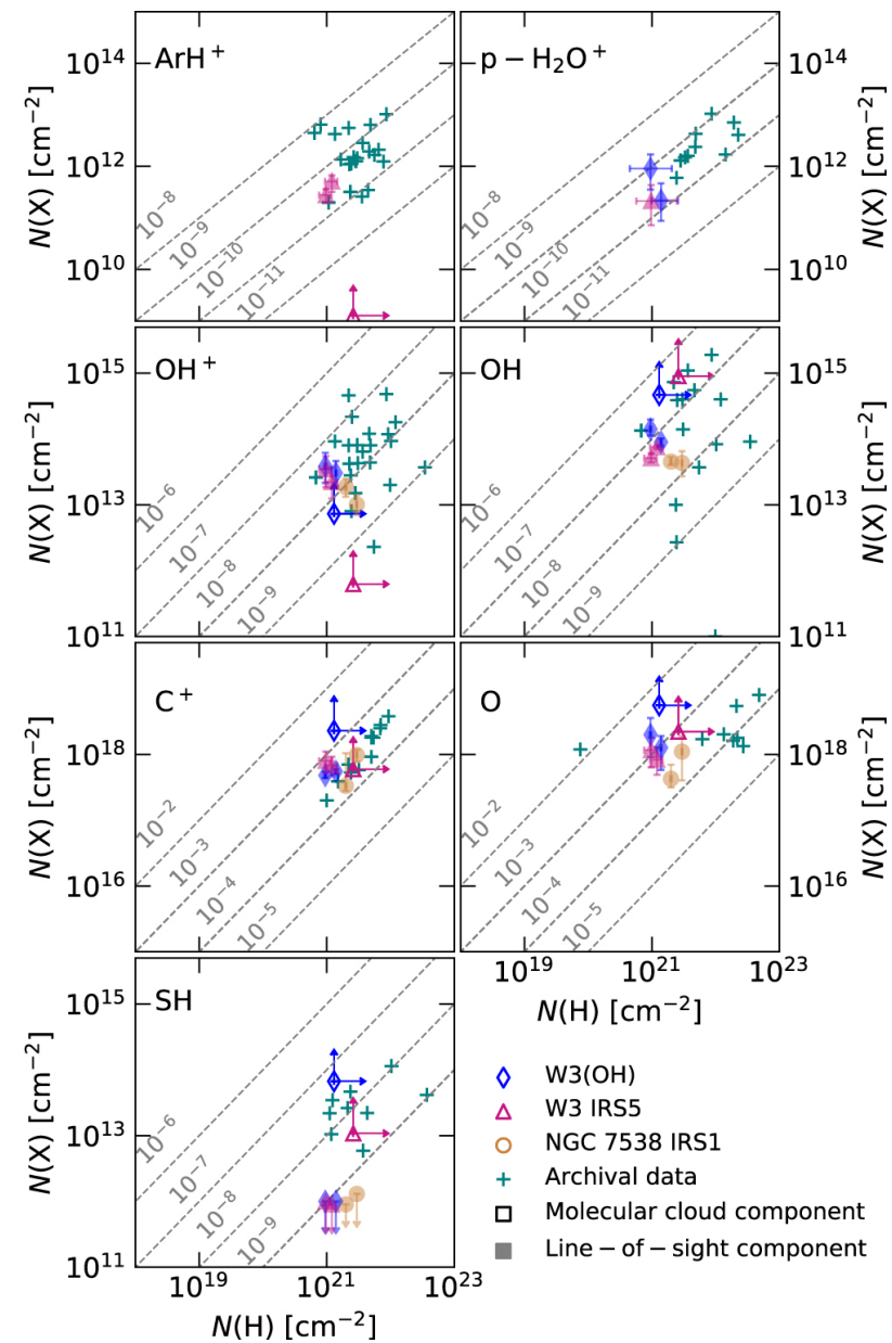
Figure 12. from A. M. Jacob et al 2022 Astrophys. J. 930 doi:10.3847/1538-4357/ac5409 https://dx.doi.org/10.3847/1538-4357/ac5409 © 2022. The Author(s). Published by the American Astronomical Society.
