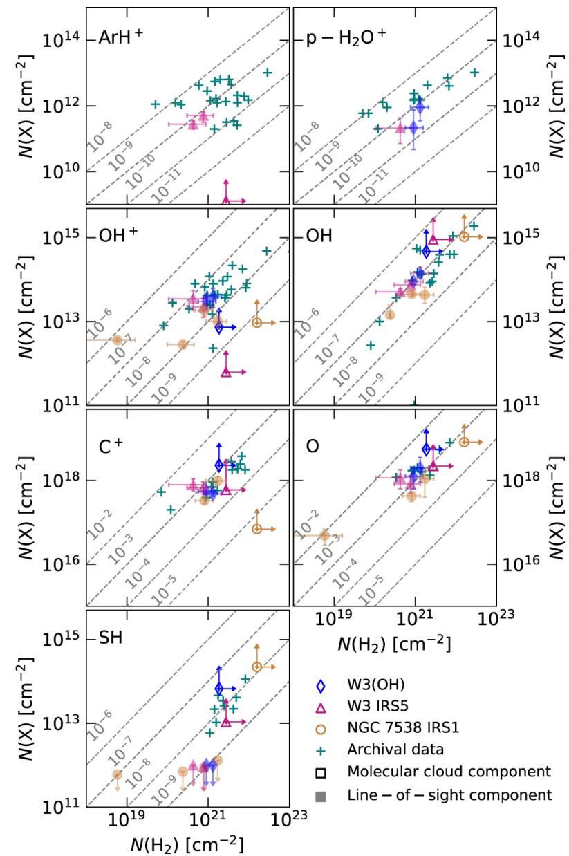
Figure 11. from A. M. Jacob et al 2022 Astrophys. J. 930 doi:10.3847/1538-4357/ac5409 https://dx.doi.org/10.3847/1538-4357/ac5409 © 2022. The Author(s). Published by the American Astronomical Society.
