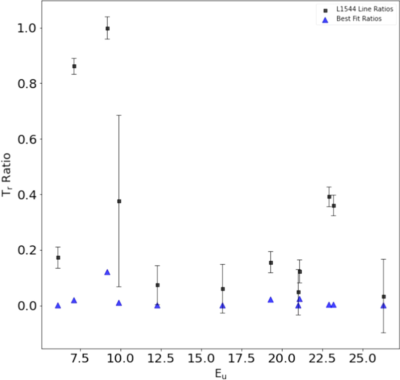
Figure 8. from UCLCHEMCMC: An MCMC Inference Tool for Physical Parameters of Molecular Clouds null 2022 APJ 927 203 doi:10.3847/1538-4357/ac51d0 https://dx.doi.org/10.3847/1538-4357/ac51d0 © 2022. The Author(s). Published by the American Astronomical Society.
