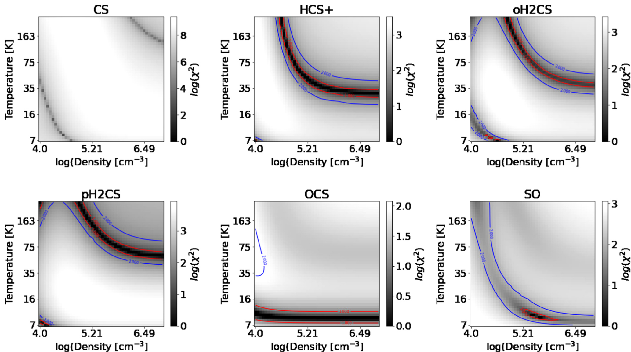
Figure 7. from UCLCHEMCMC: An MCMC Inference Tool for Physical Parameters of Molecular Clouds null 2022 APJ 927 203 doi:10.3847/1538-4357/ac51d0 https://dx.doi.org/10.3847/1538-4357/ac51d0 © 2022. The Author(s). Published by the American Astronomical Society.
