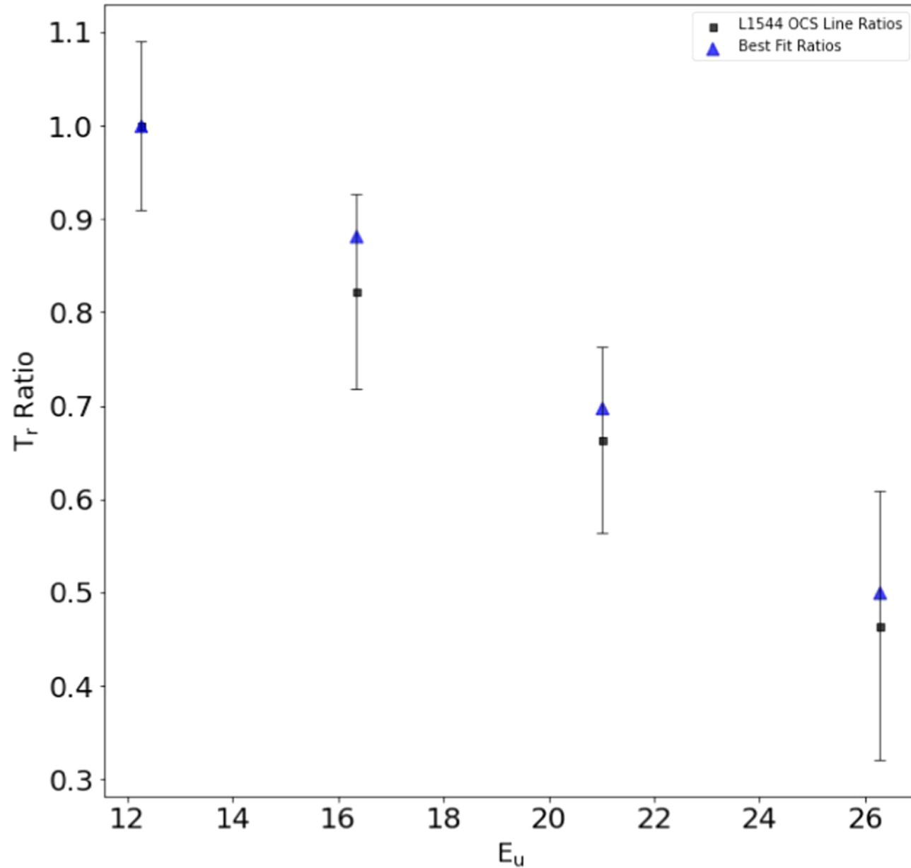
Figure 6. from UCLCHEMCMC: An MCMC Inference Tool for Physical Parameters of Molecular Clouds null 2022 APJ 927 203 doi:10.3847/1538-4357/ac51d0 https://dx.doi.org/10.3847/1538-4357/ac51d0 © 2022. The Author(s). Published by the American Astronomical Society.
