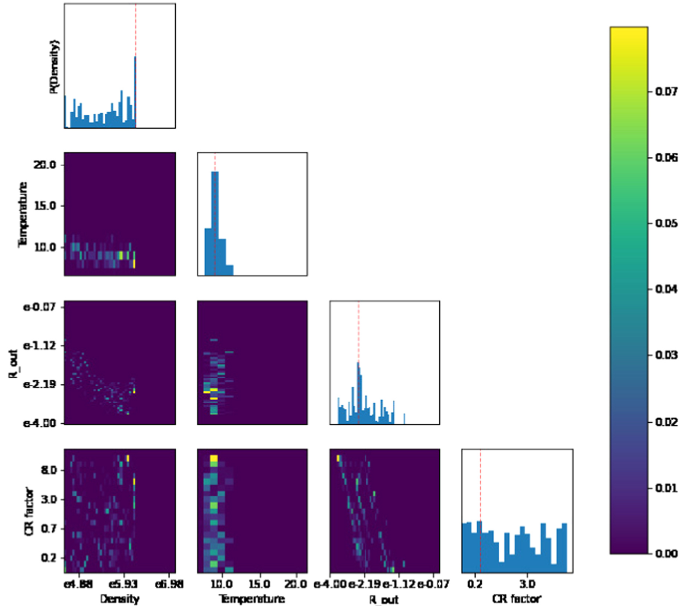
Figure 5. from UCLCHEMCMC: An MCMC Inference Tool for Physical Parameters of Molecular Clouds null 2022 APJ 927 203 doi:10.3847/1538-4357/ac51d0 https://dx.doi.org/10.3847/1538-4357/ac51d0 © 2022. The Author(s). Published by the American Astronomical Society.
