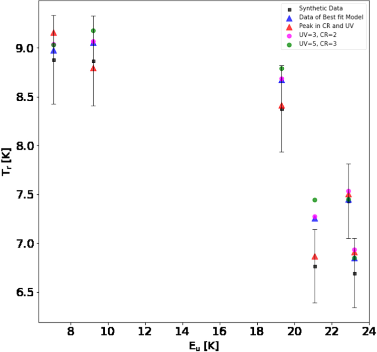
Figure 4. from UCLCHEMCMC: An MCMC Inference Tool for Physical Parameters of Molecular Clouds null 2022 APJ 927 203 doi:10.3847/1538-4357/ac51d0 https://dx.doi.org/10.3847/1538-4357/ac51d0 © 2022. The Author(s). Published by the American Astronomical Society.
