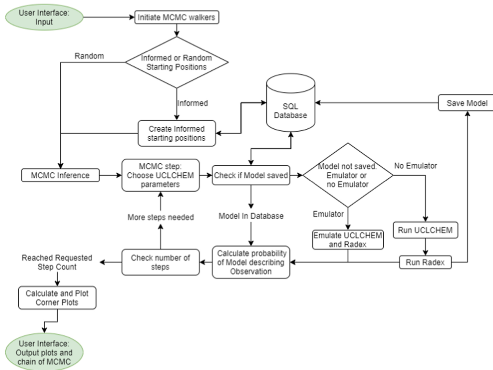
Figure 1. from UCLCHEMCMC: An MCMC Inference Tool for Physical Parameters of Molecular Clouds null 2022 APJ 927 203 doi:10.3847/1538-4357/ac51d0 https://dx.doi.org/10.3847/1538-4357/ac51d0 © 2022. The Author(s). Published by the American Astronomical Society.
