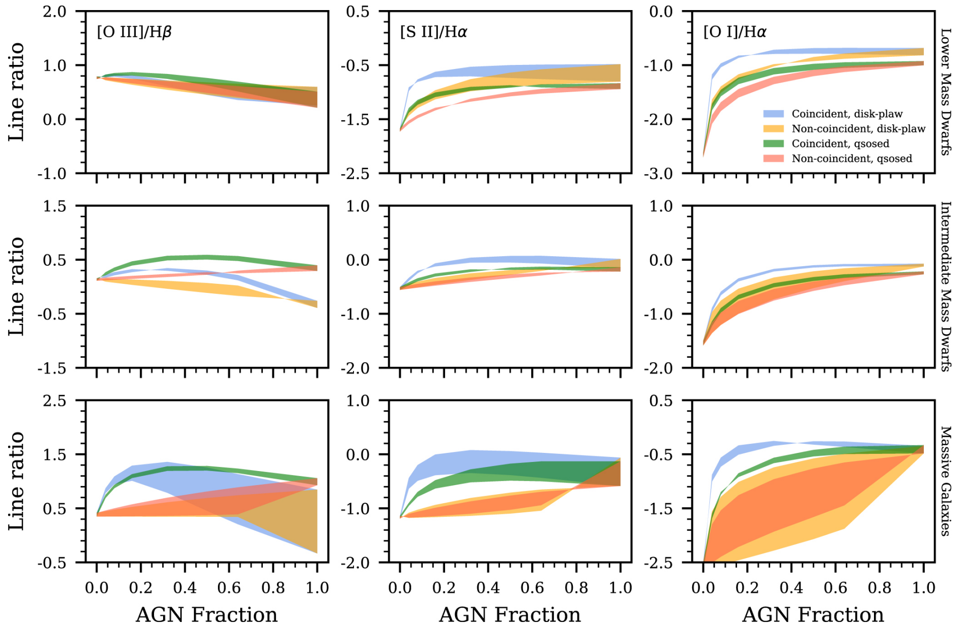
Figure 4. from Chris T. Richardson et al 2022 Astrophys. J. 927 doi:10.3847/1538-4357/ac510c https://dx.doi.org/10.3847/1538-4357/ac510c © 2022. The Author(s). Published by the American Astronomical Society.
