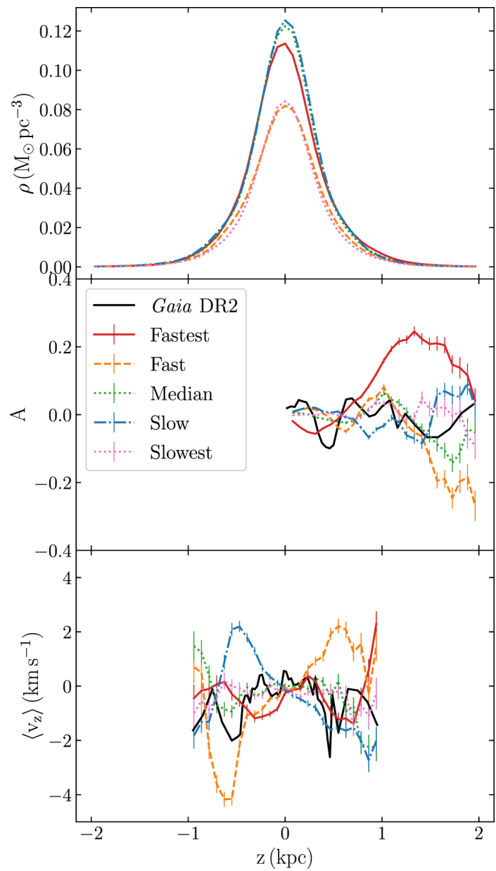
Figure 6. from Morgan Bennett et al 2022 Astrophys. J. 927 doi:10.3847/1538-4357/ac5021 https://dx.doi.org/10.3847/1538-4357/ac5021 © 2022. The Author(s). Published by the American Astronomical Society.
