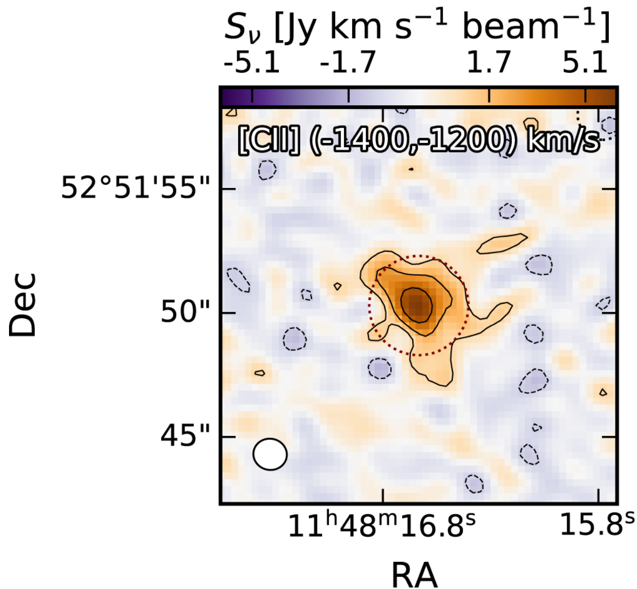
Figure 22. from Physical Constraints on the Extended Interstellar Medium of the z = 6.42 Quasar J1148+5251: [C II]158 m, [N II]205 m, and [O I]146 m Observations null 2022 APJ 927 152 doi:10.3847/1538-4357/ac4e94 https://dx.doi.org/10.3847/1538-4357/ac4e94 © 2022. The Author(s). Published by the American Astronomical Society.
