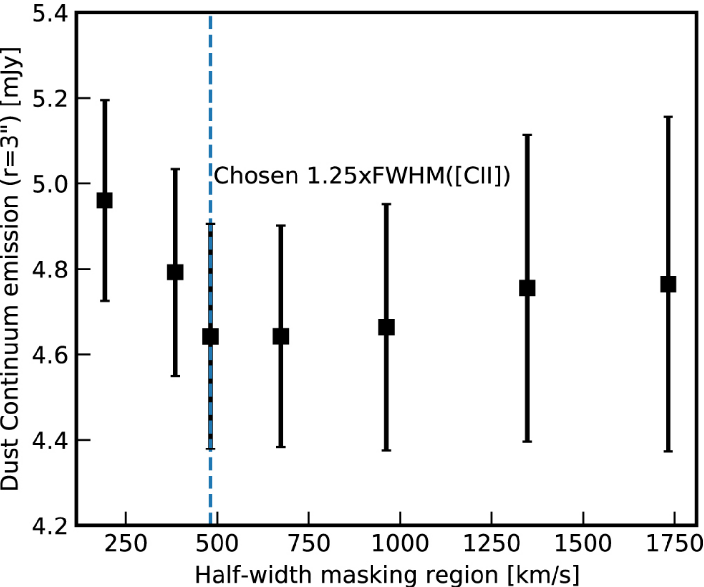
Figure 18. from Physical Constraints on the Extended Interstellar Medium of the z = 6.42 Quasar J1148+5251: [C II]158 m, [N II]205 m, and [O I]146 m Observations null 2022 APJ 927 152 doi:10.3847/1538-4357/ac4e94 https://dx.doi.org/10.3847/1538-4357/ac4e94 © 2022. The Author(s). Published by the American Astronomical Society.
