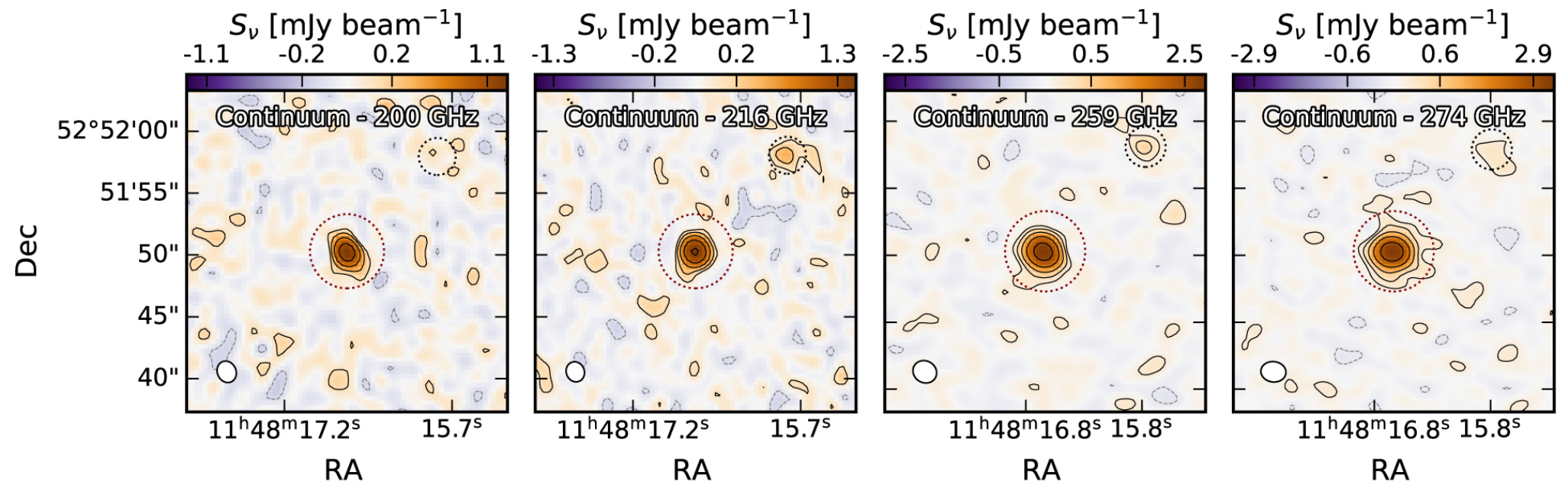
Figure 1. from Physical Constraints on the Extended Interstellar Medium of the z = 6.42 Quasar J1148+5251: [C II]158 m, [N II]205 m, and [O I]146 m Observations null 2022 APJ 927 152 doi:10.3847/1538-4357/ac4e94 https://dx.doi.org/10.3847/1538-4357/ac4e94 © 2022. The Author(s). Published by the American Astronomical Society.
