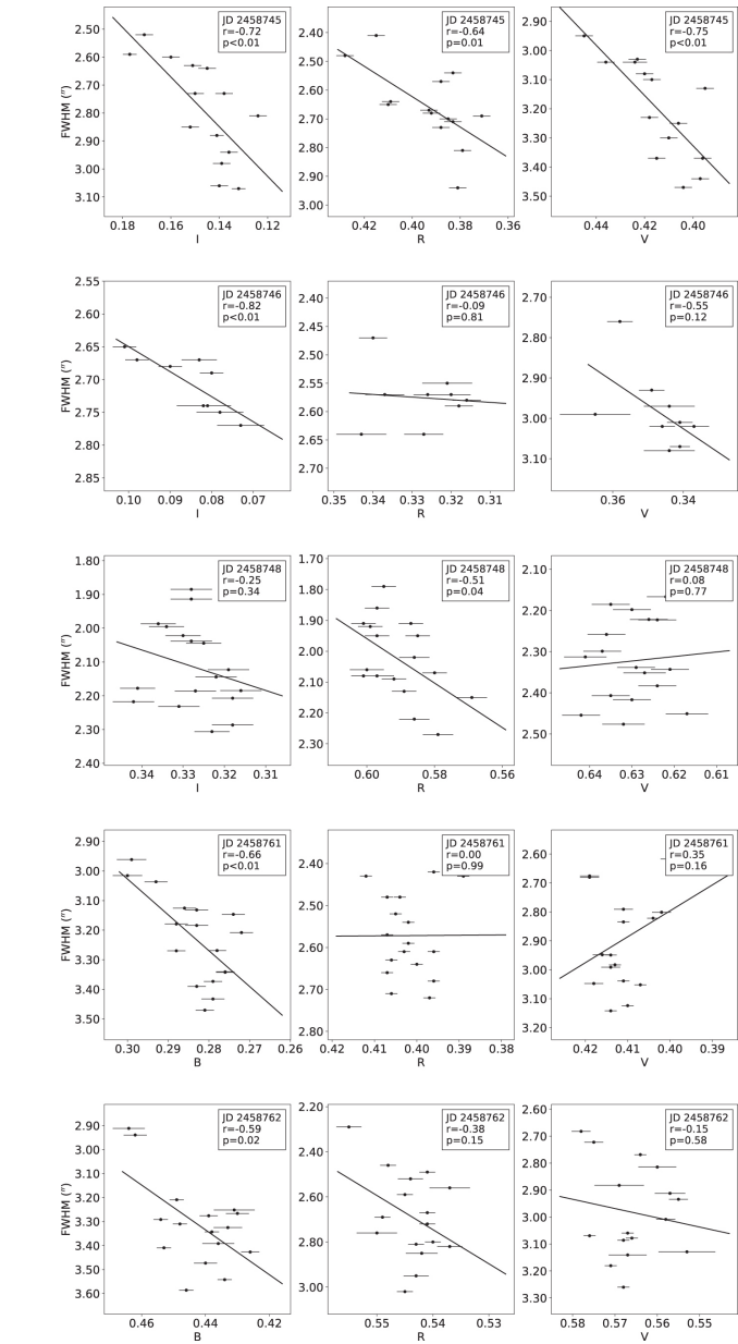
Figure 4. from Intraday Optical Multiband Observation of BL Lacertae null 2022 APJ 926 91 doi:10.3847/1538-4357/ac4490 https://dx.doi.org/10.3847/1538-4357/ac4490 © 2022. The Author(s). Published by the American Astronomical Society.
