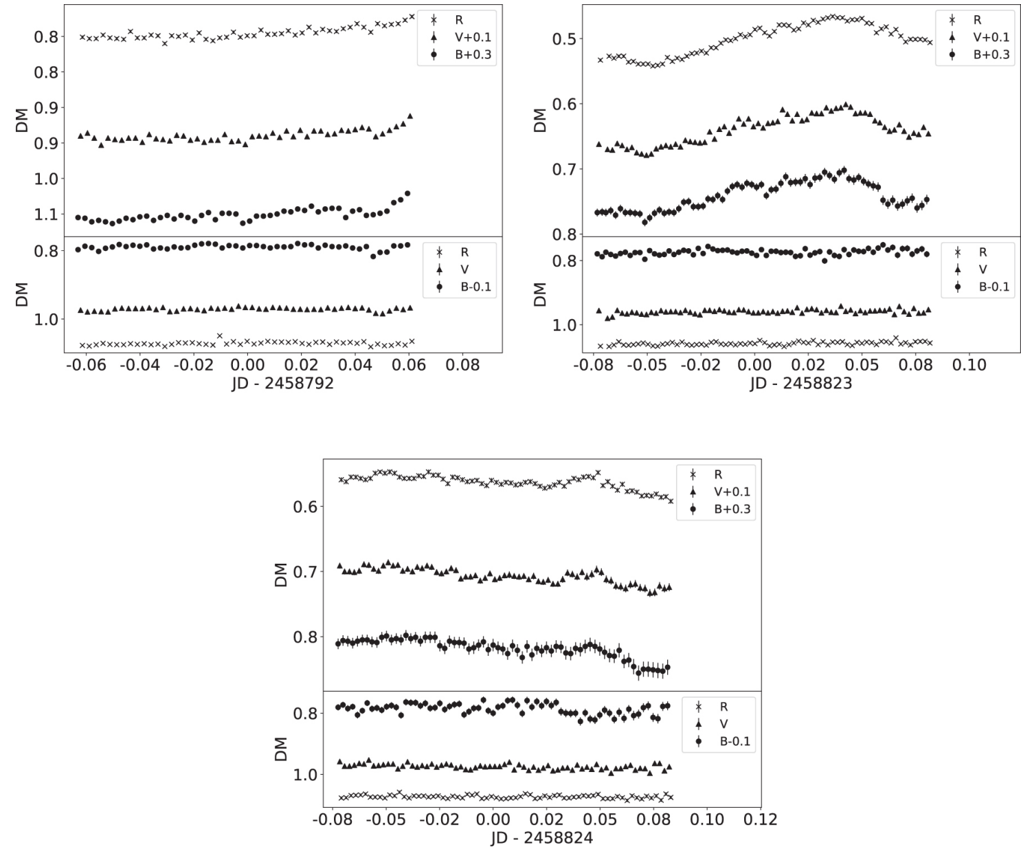
Figure 3. from Intraday Optical Multiband Observation of BL Lacertae null 2022 APJ 926 91 doi:10.3847/1538-4357/ac4490 https://dx.doi.org/10.3847/1538-4357/ac4490 © 2022. The Author(s). Published by the American Astronomical Society.
