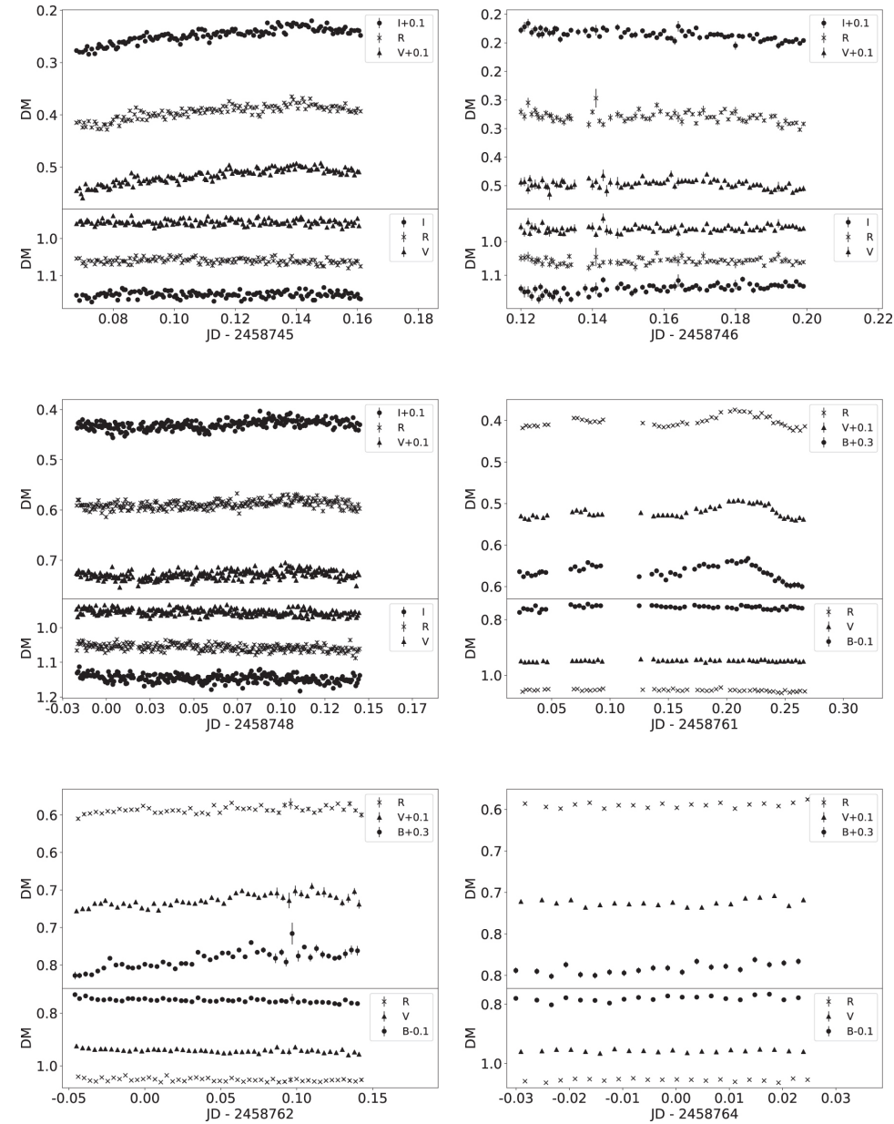
Figure 3. from Intraday Optical Multiband Observation of BL Lacertae null 2022 APJ 926 91 doi:10.3847/1538-4357/ac4490 https://dx.doi.org/10.3847/1538-4357/ac4490 © 2022. The Author(s). Published by the American Astronomical Society.
