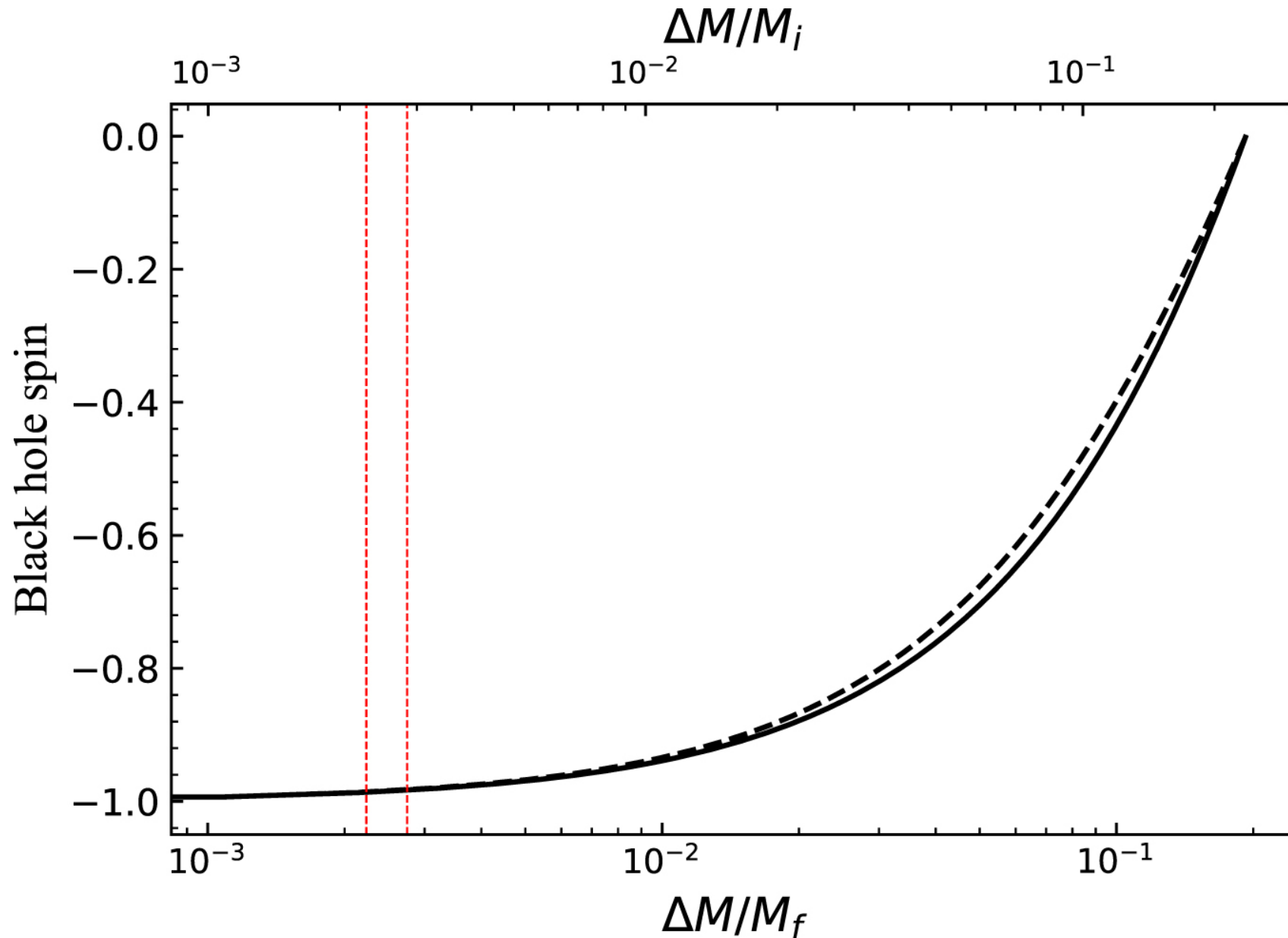
Figure 8. from Estimating the Spin of the Black Hole Candidate MAXI J1659-152 with the X-Ray Continuum-fitting Method null 2022 APJ 925 142 doi:10.3847/1538-4357/ac4163 https://dx.doi.org/10.3847/1538-4357/ac4163 © 2022. The Author(s). Published by the American Astronomical Society.
