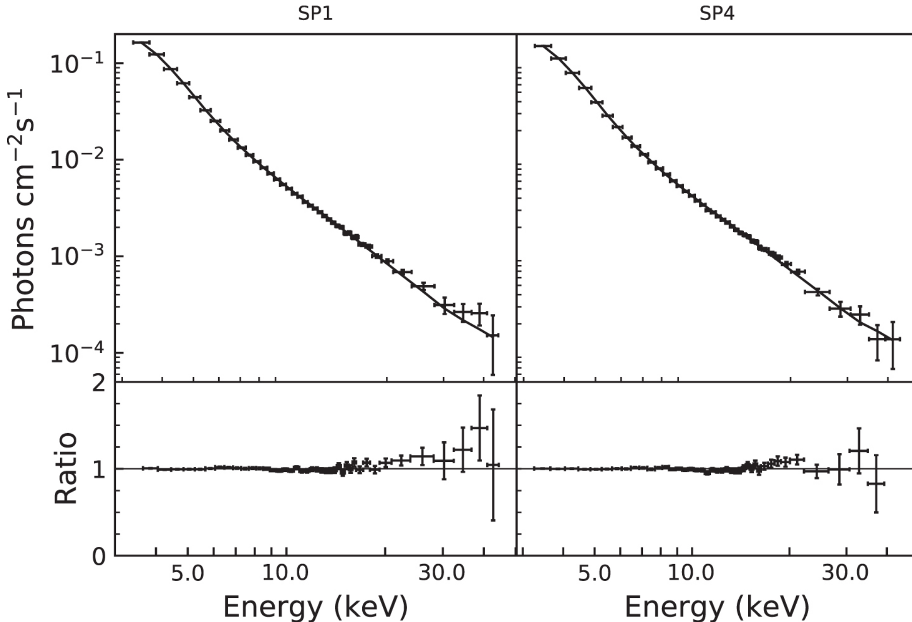
Figure 3. from Estimating the Spin of the Black Hole Candidate MAXI J1659-152 with the X-Ray Continuum-fitting Method null 2022 APJ 925 142 doi:10.3847/1538-4357/ac4163 https://dx.doi.org/10.3847/1538-4357/ac4163 © 2022. The Author(s). Published by the American Astronomical Society.
