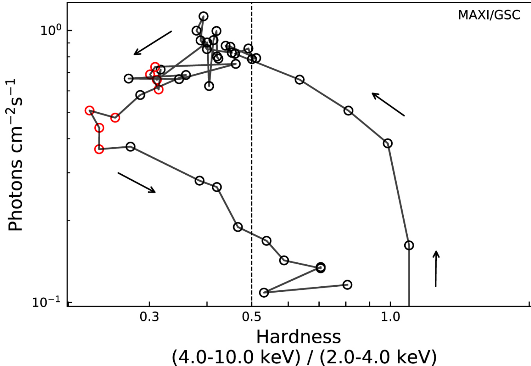
Figure 2. from Estimating the Spin of the Black Hole Candidate MAXI J1659-152 with the X-Ray Continuum-fitting Method null 2022 APJ 925 142 doi:10.3847/1538-4357/ac4163 https://dx.doi.org/10.3847/1538-4357/ac4163 © 2022. The Author(s). Published by the American Astronomical Society.
