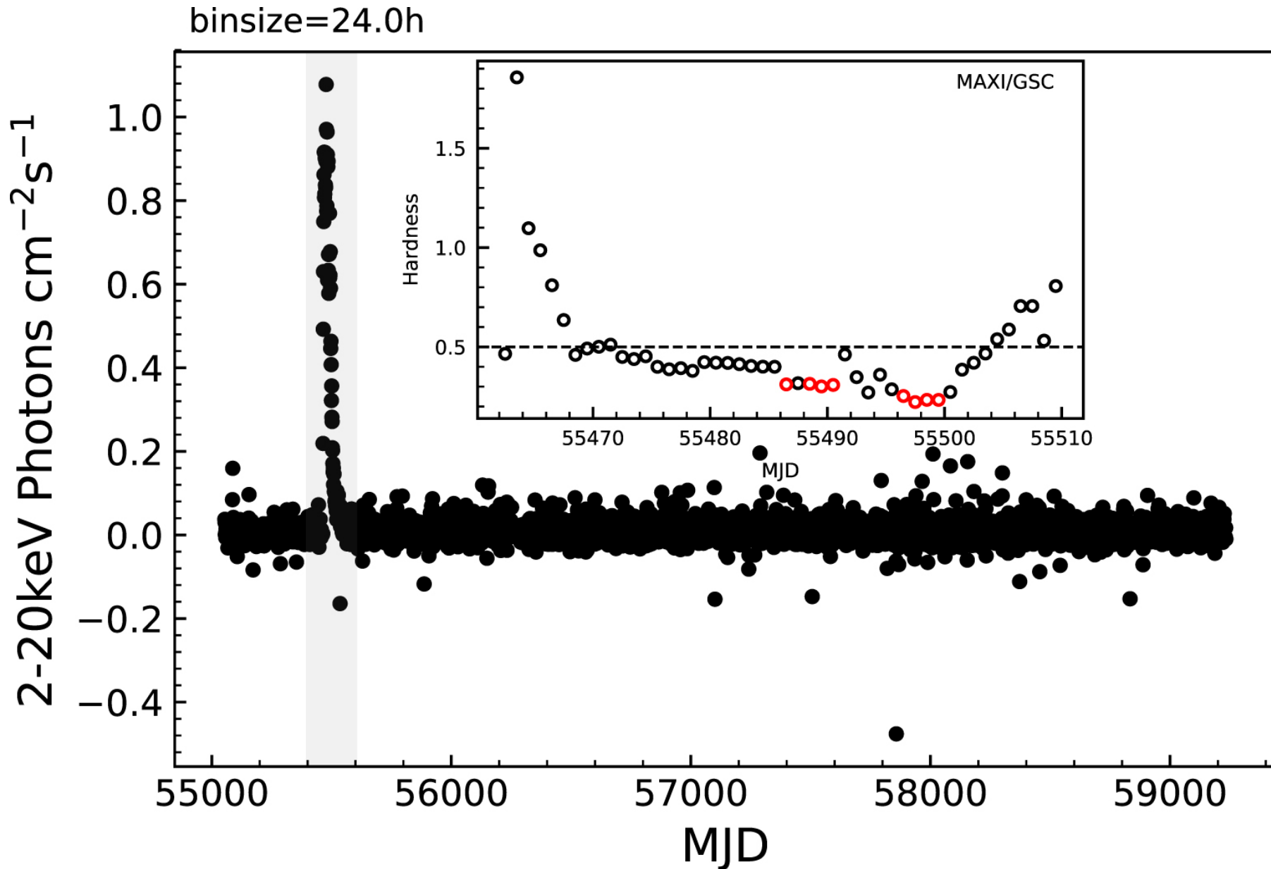
Figure 1. from Estimating the Spin of the Black Hole Candidate MAXI J1659-152 with the X-Ray Continuum-fitting Method null 2022 APJ 925 142 doi:10.3847/1538-4357/ac4163 https://dx.doi.org/10.3847/1538-4357/ac4163 © 2022. The Author(s). Published by the American Astronomical Society.
