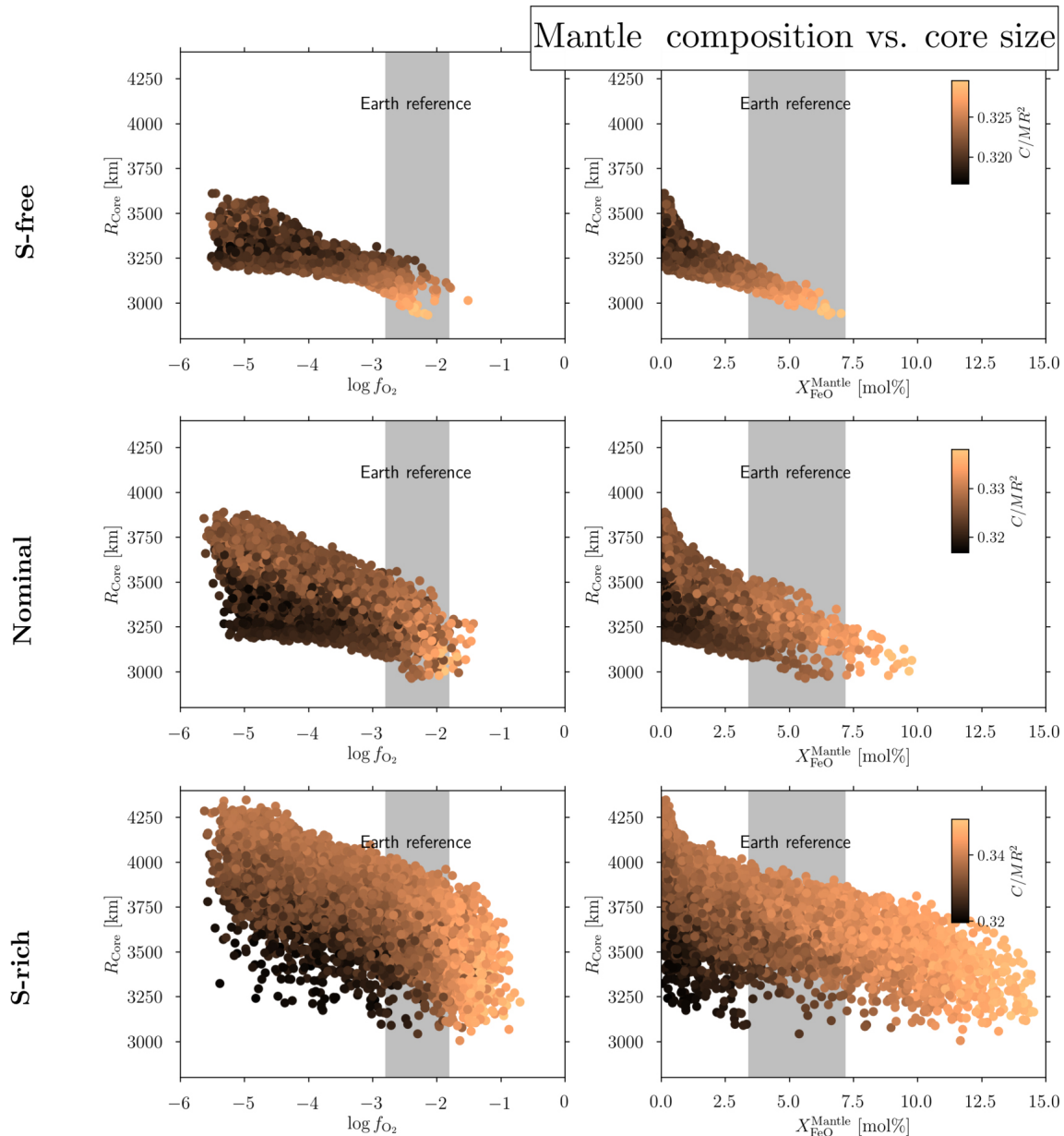
Figure 8. from Possible Chemical Composition And Interior Structure Models Of Venus Inferred From Numerical Modelling null 2022 APJ 926 217 doi:10.3847/1538-4357/ac410d https://dx.doi.org/10.3847/1538-4357/ac410d © 2022. The Author(s). Published by the American Astronomical Society.
