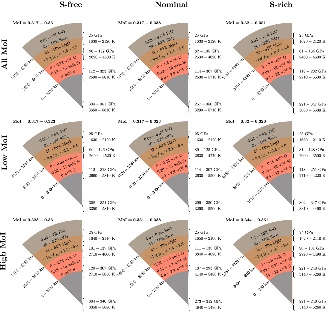
Figure 7. from Possible Chemical Composition And Interior Structure Models Of Venus Inferred From Numerical Modelling null 2022 APJ 926 217 doi:10.3847/1538-4357/ac410d https://dx.doi.org/10.3847/1538-4357/ac410d © 2022. The Author(s). Published by the American Astronomical Society.
