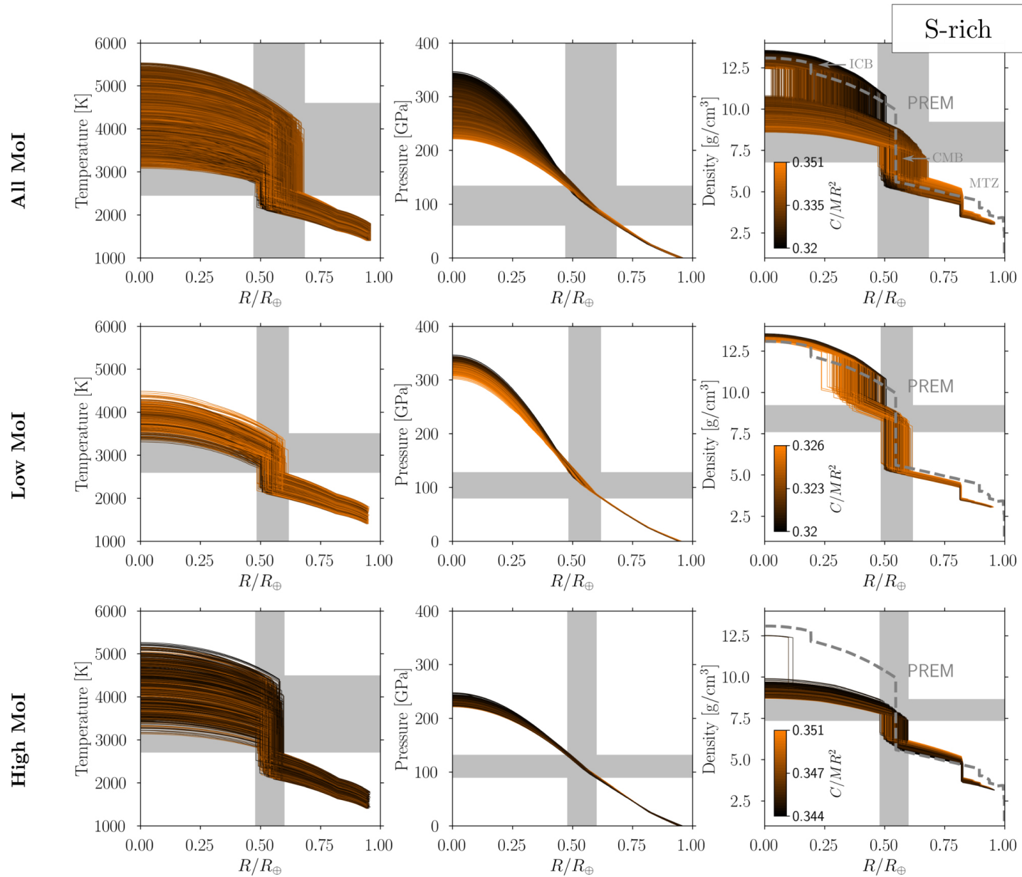
Figure 6. from Possible Chemical Composition And Interior Structure Models Of Venus Inferred From Numerical Modelling null 2022 APJ 926 217 doi:10.3847/1538-4357/ac410d https://dx.doi.org/10.3847/1538-4357/ac410d © 2022. The Author(s). Published by the American Astronomical Society.
