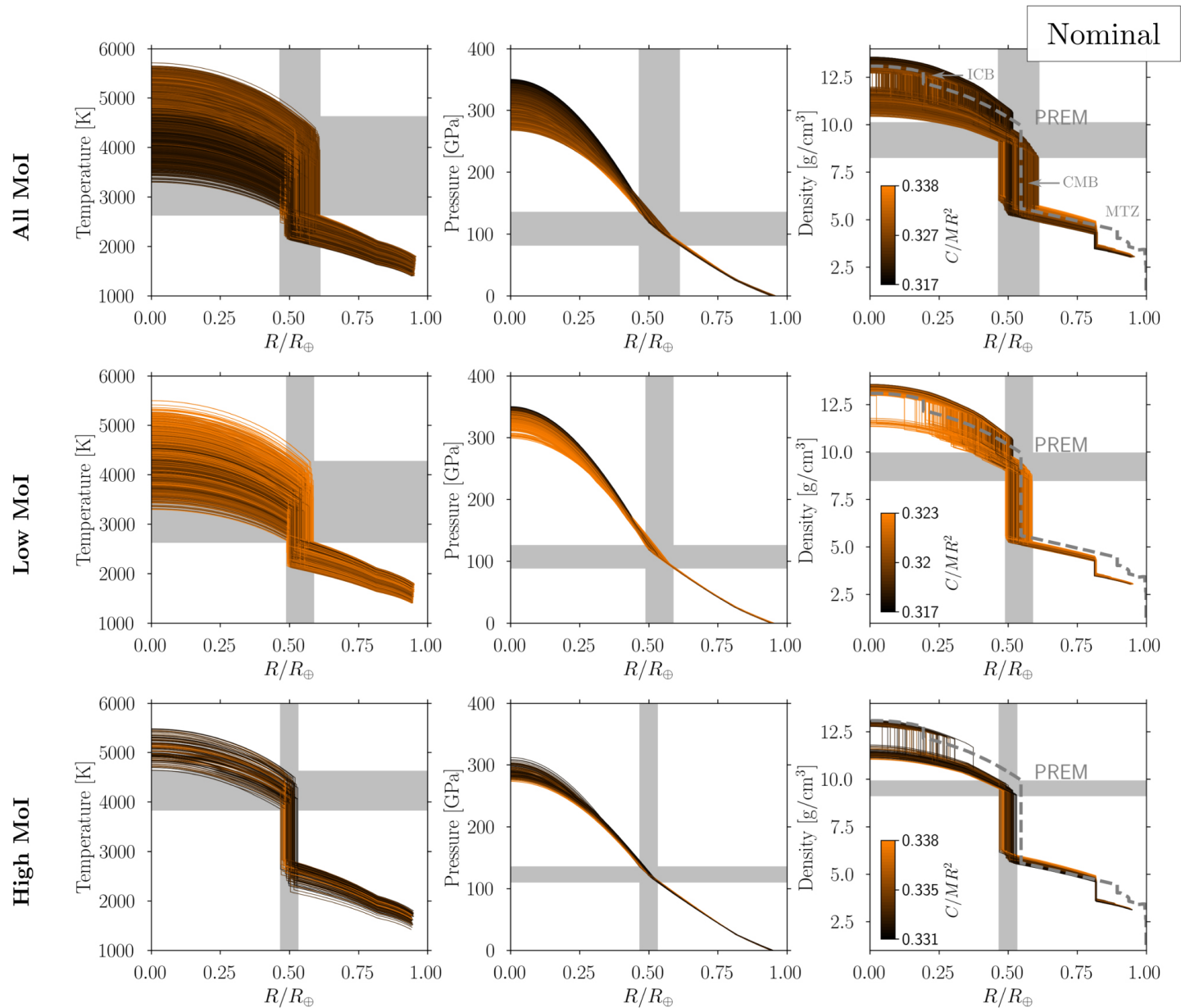
Figure 5. from Possible Chemical Composition And Interior Structure Models Of Venus Inferred From Numerical Modelling null 2022 APJ 926 217 doi:10.3847/1538-4357/ac410d https://dx.doi.org/10.3847/1538-4357/ac410d © 2022. The Author(s). Published by the American Astronomical Society.
