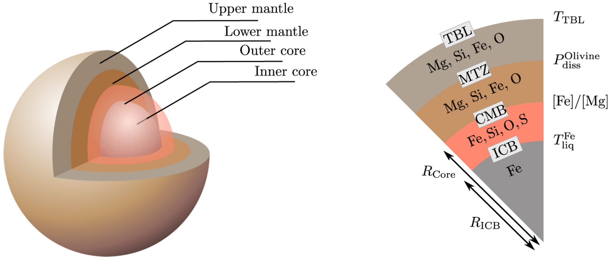
Figure 1. from Possible Chemical Composition And Interior Structure Models Of Venus Inferred From Numerical Modelling null 2022 APJ 926 217 doi:10.3847/1538-4357/ac410d https://dx.doi.org/10.3847/1538-4357/ac410d © 2022. The Author(s). Published by the American Astronomical Society.
