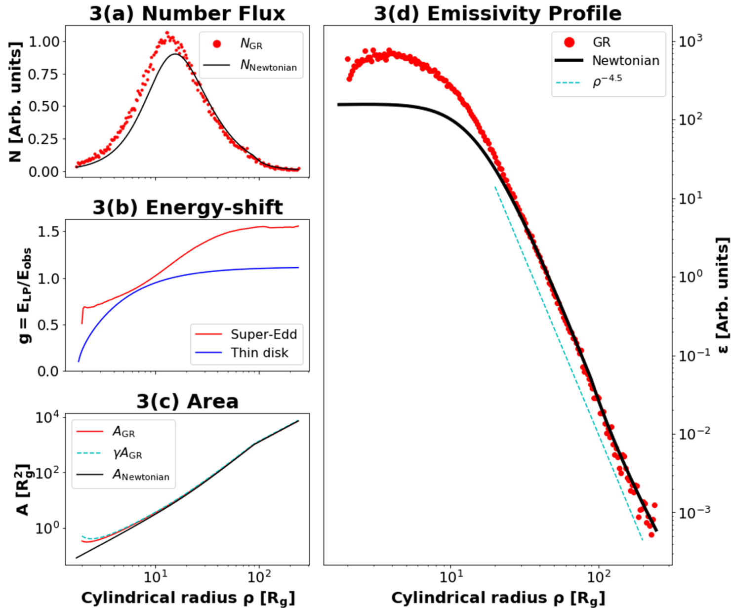
Figure 3. from Relativistic X-Ray Reverberation from Super-Eddington Accretion Flow null 2022 APJ 925 151 doi:10.3847/1538-4357/ac3df3 https://dx.doi.org/10.3847/1538-4357/ac3df3
