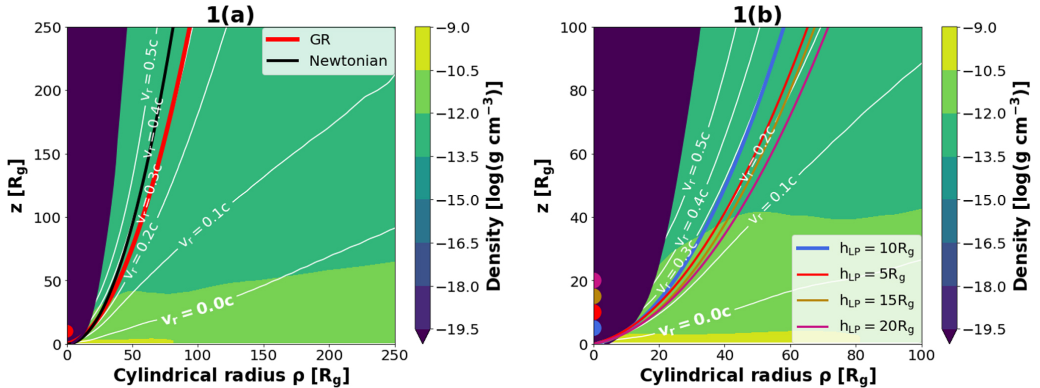
Figure 1. from Relativistic X-Ray Reverberation from Super-Eddington Accretion Flow null 2022 APJ 925 151 doi:10.3847/1538-4357/ac3df3 https://dx.doi.org/10.3847/1538-4357/ac3df3 © 2022. The Author(s). Published by the American Astronomical Society.
