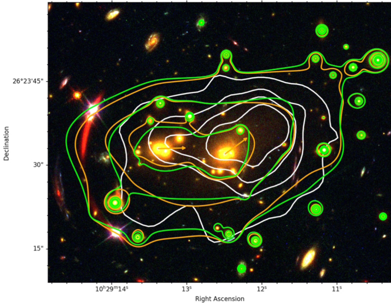
Figure 8. from VLT/MUSE Observations of SDSS J1029+2623: Toward a High-precision Strong Lensing Model null 2022 APJ 926 86 doi:10.3847/1538-4357/ac3d35 https://dx.doi.org/10.3847/1538-4357/ac3d35 © 2022. The Author(s). Published by the American Astronomical Society.
