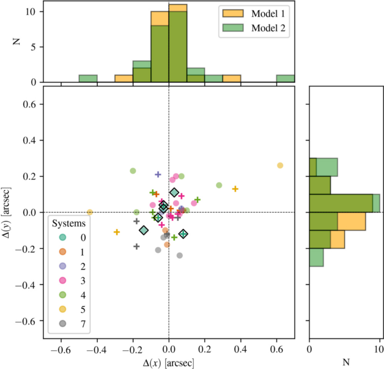
Figure 6. from VLT/MUSE Observations of SDSS J1029+2623: Toward a High-precision Strong Lensing Model null 2022 APJ 926 86 doi:10.3847/1538-4357/ac3d35 https://dx.doi.org/10.3847/1538-4357/ac3d35 © 2022. The Author(s). Published by the American Astronomical Society.
