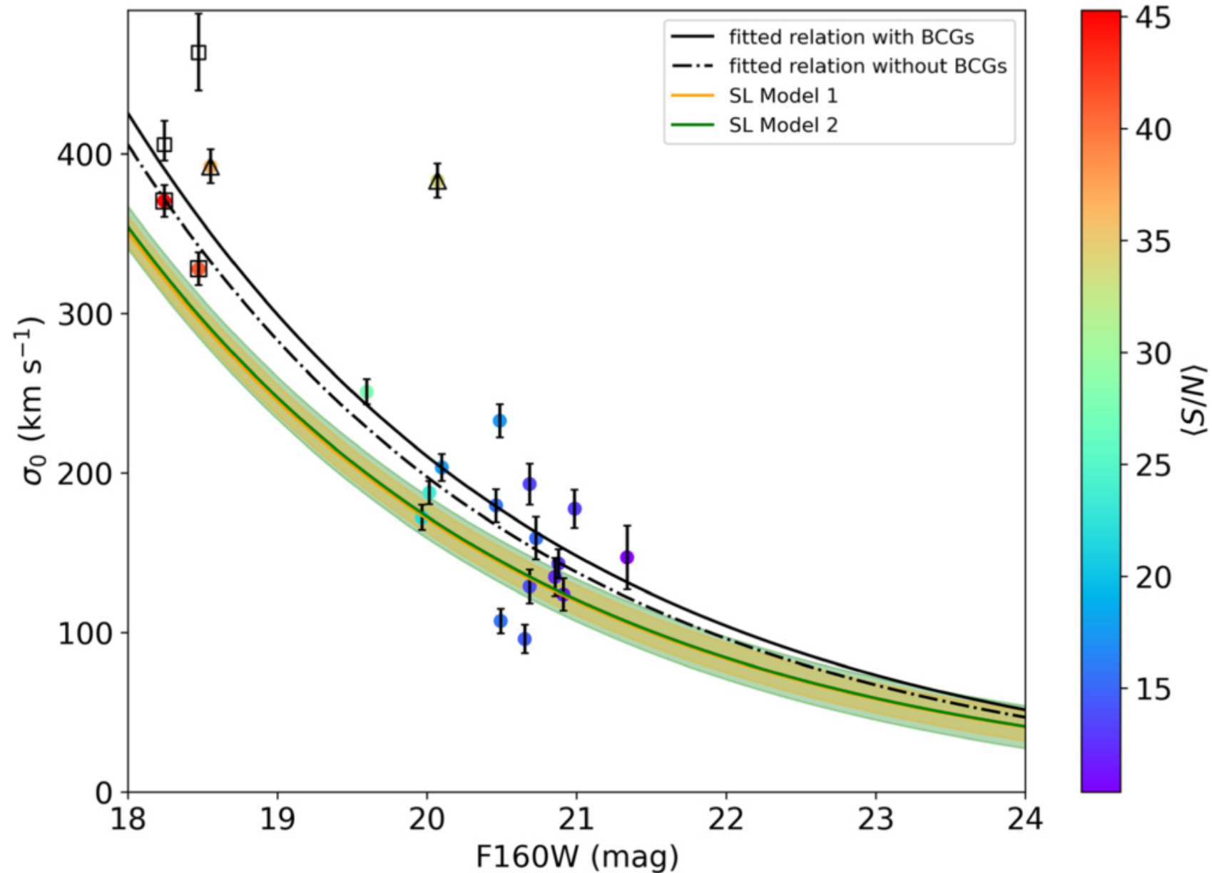
Figure 5. from VLT/MUSE Observations of SDSS J1029+2623: Toward a High-precision Strong Lensing Model null 2022 APJ 926 86 doi:10.3847/1538-4357/ac3d35 https://dx.doi.org/10.3847/1538-4357/ac3d35 © 2022. The Author(s). Published by the American Astronomical Society.
