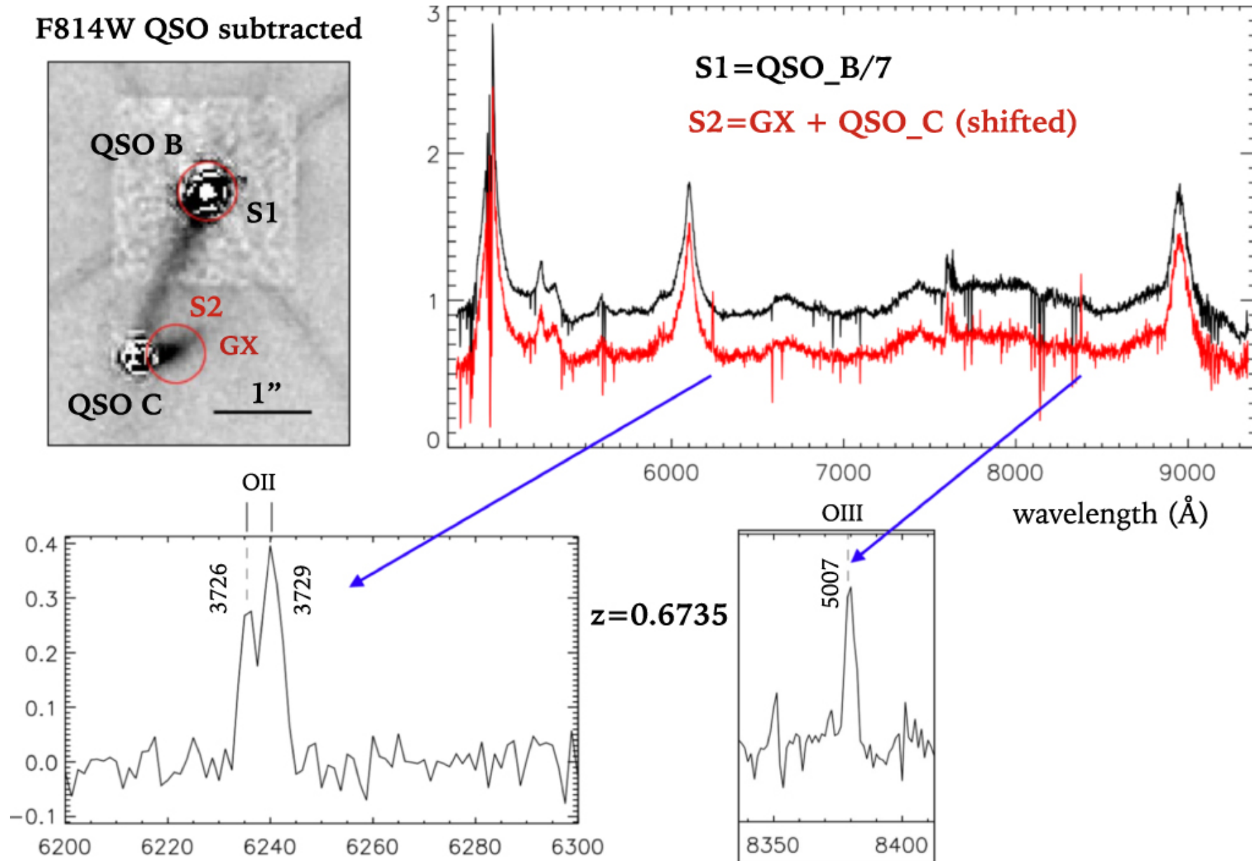
Figure 4. from VLT/MUSE Observations of SDSS J1029+2623: Toward a High-precision Strong Lensing Model null 2022 APJ 926 86 doi:10.3847/1538-4357/ac3d35 https://dx.doi.org/10.3847/1538-4357/ac3d35 © 2022. The Author(s). Published by the American Astronomical Society.
