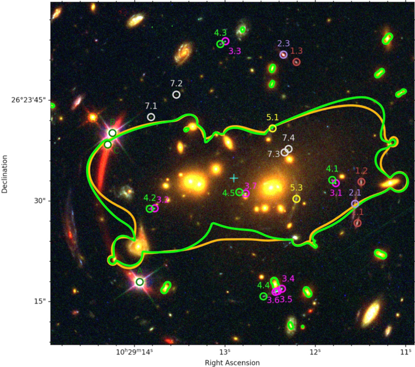
Figure 3. from VLT/MUSE Observations of SDSS J1029+2623: Toward a High-precision Strong Lensing Model null 2022 APJ 926 86 doi:10.3847/1538-4357/ac3d35 https://dx.doi.org/10.3847/1538-4357/ac3d35 © 2022. The Author(s). Published by the American Astronomical Society.
