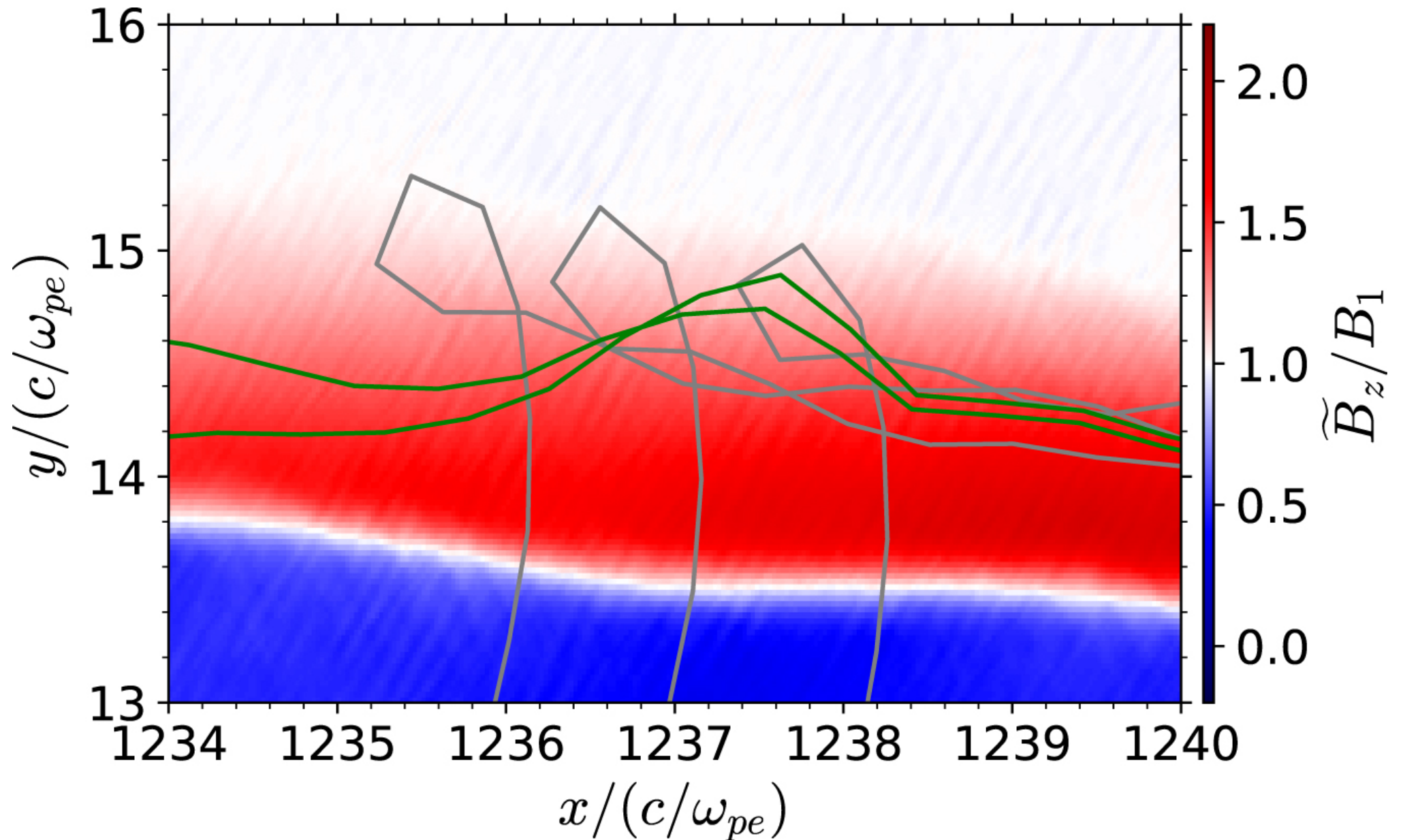
Figure 8. from Particle Acceleration by Pickup Process Upstream of Relativistic Shocks null 2022 APJ 924 108 doi:10.3847/1538-4357/ac38aa https://dx.doi.org/10.3847/1538-4357/ac38aa © 2022. The Author(s). Published by the American Astronomical Society.
