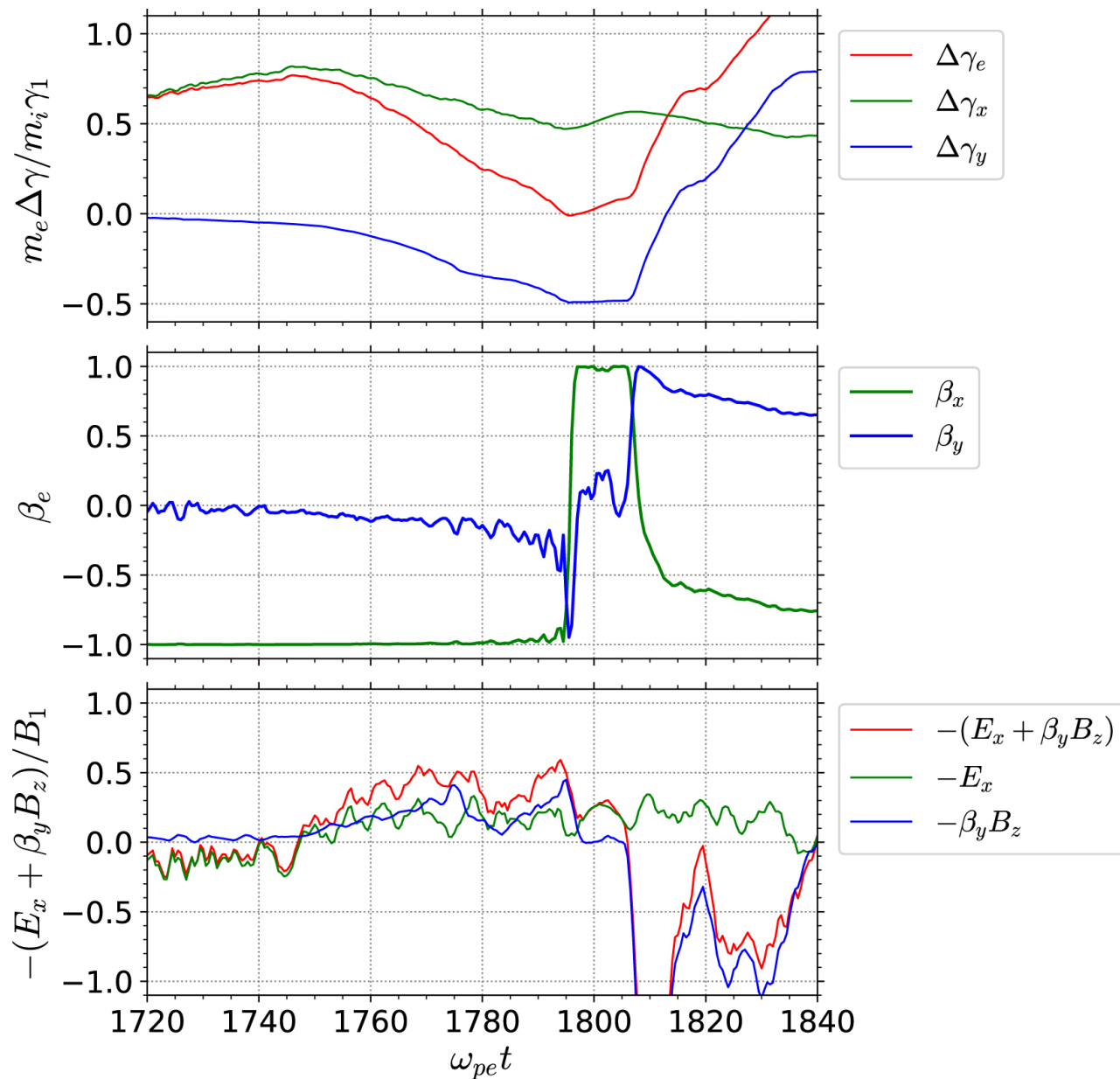
Figure 6. from Particle Acceleration by Pickup Process Upstream of Relativistic Shocks null 2022 APJ 924 108 doi:10.3847/1538-4357/ac38aa https://dx.doi.org/10.3847/1538-4357/ac38aa
