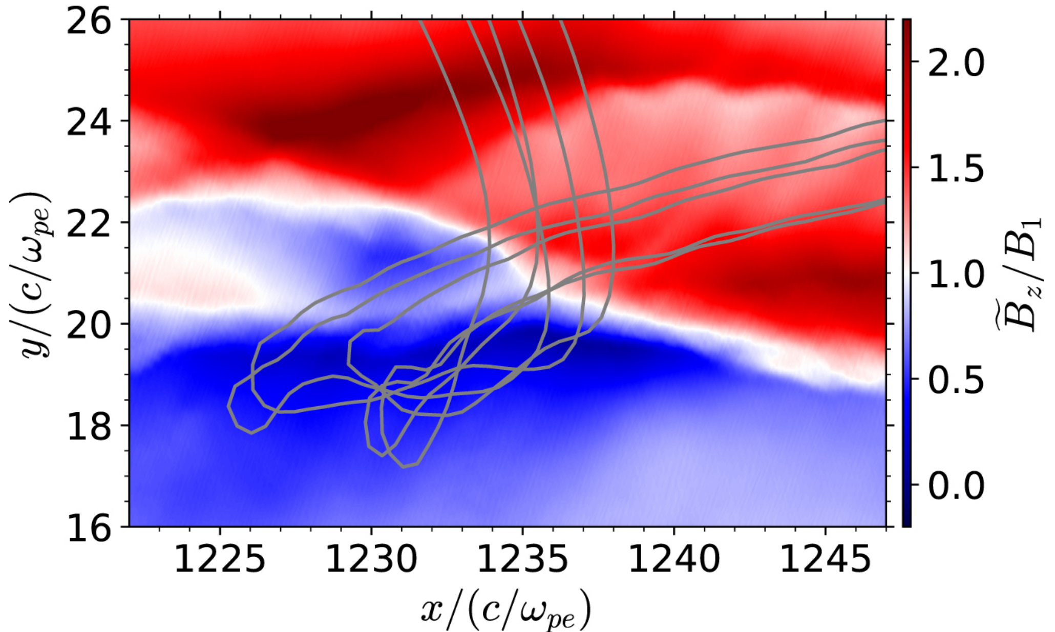
Figure 5. from Particle Acceleration by Pickup Process Upstream of Relativistic Shocks null 2022 APJ 924 108 doi:10.3847/1538-4357/ac38aa https://dx.doi.org/10.3847/1538-4357/ac38aa © 2022. The Author(s). Published by the American Astronomical Society.
