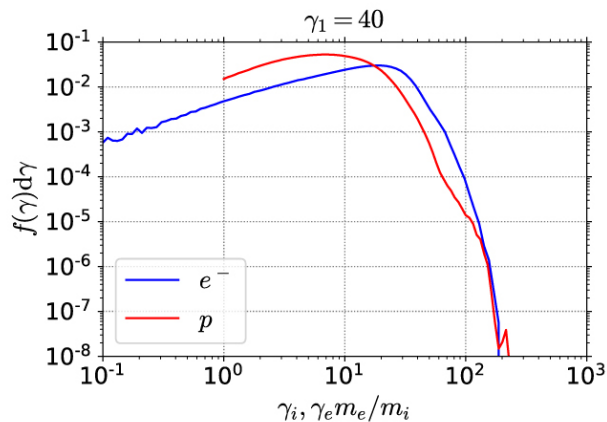
(a) 700 \leq x/(c/\omega_{pe}) \leq 1050
