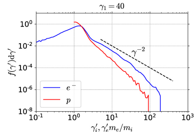
(c) measured in the proper frame
