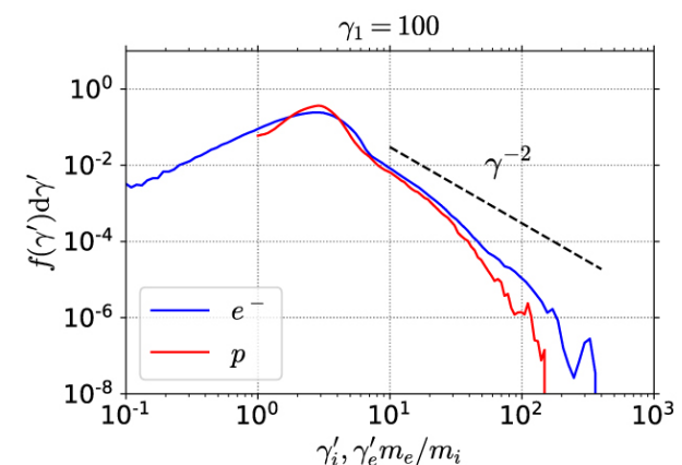
(f) measured in the proper frame
