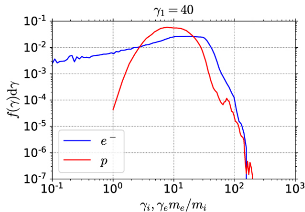
(b) 1120 \leq x/(c/\omega_{pe}) \leq 1200
