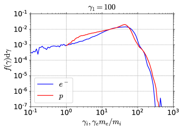
(e) 1120 \leq x/(c/\omega_{pe}) \leq 1200
