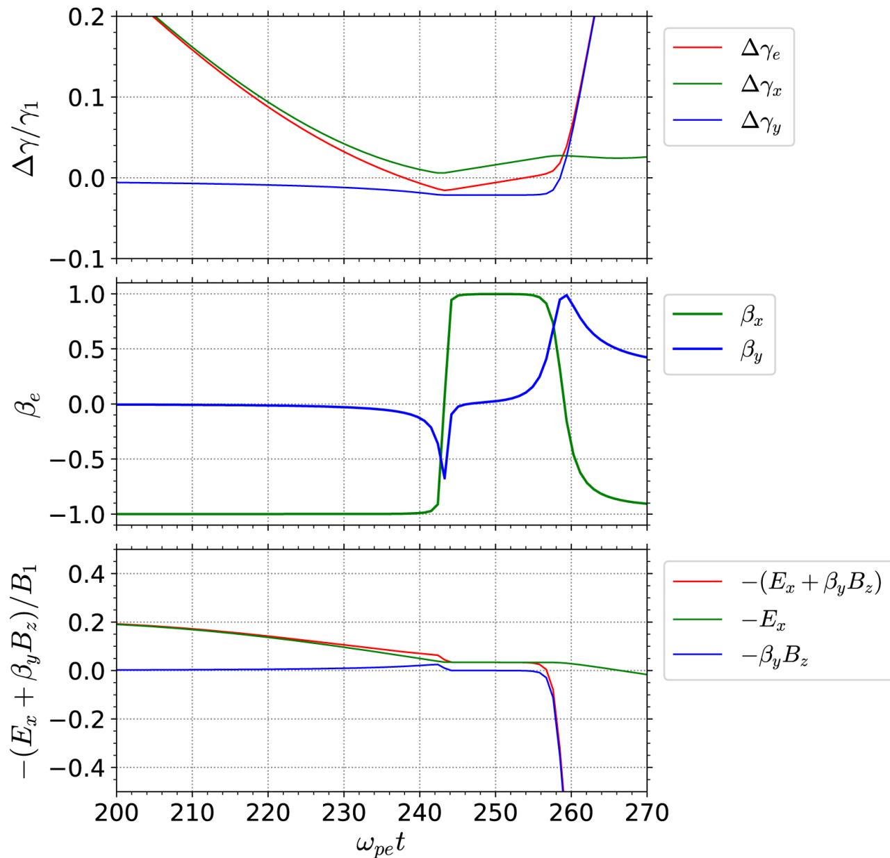
Figure 12. from Particle Acceleration by Pickup Process Upstream of Relativistic Shocks null 2022 APJ 924 108 doi:10.3847/1538-4357/ac38aa https://dx.doi.org/10.3847/1538-4357/ac38aa
