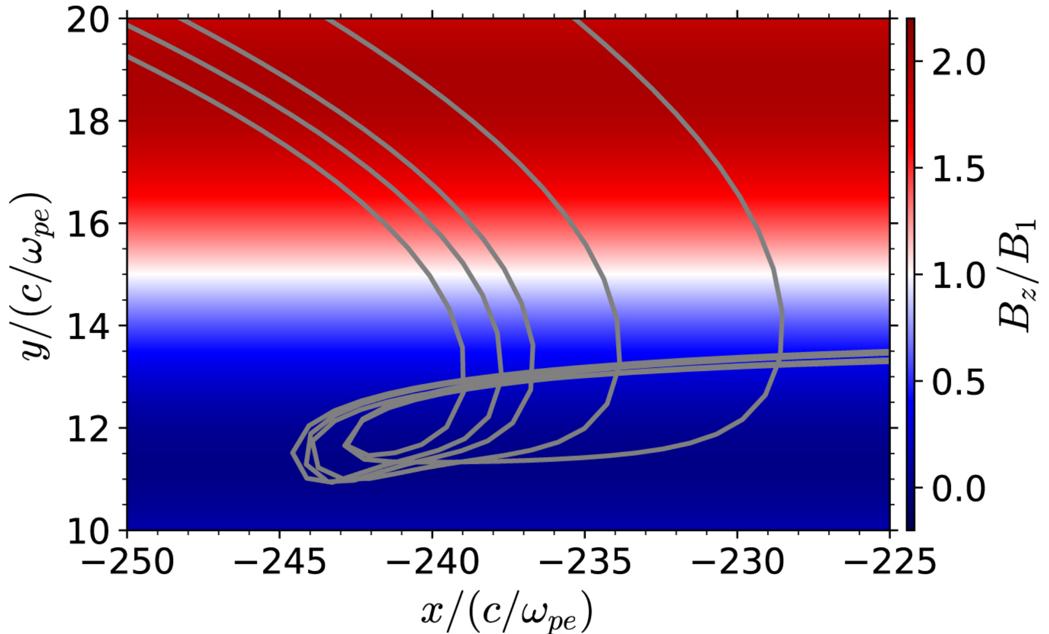
Figure 11. from Particle Acceleration by Pickup Process Upstream of Relativistic Shocks null 2022 APJ 924 108 doi:10.3847/1538-4357/ac38aa https://dx.doi.org/10.3847/1538-4357/ac38aa © 2022. The Author(s). Published by the American Astronomical Society.
