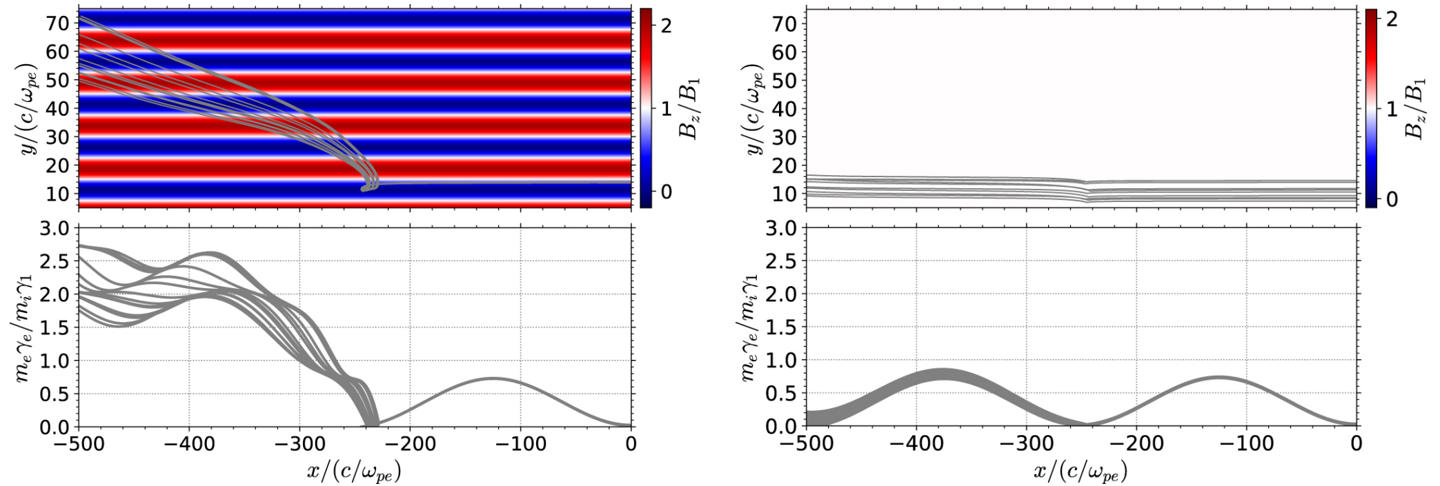
Figure 10. from Particle Acceleration by Pickup Process Upstream of Relativistic Shocks null 2022 APJ 924 108 doi:10.3847/1538-4357/ac38aa https://dx.doi.org/10.3847/1538-4357/ac38aa © 2022. The Author(s). Published by the American Astronomical Society.
