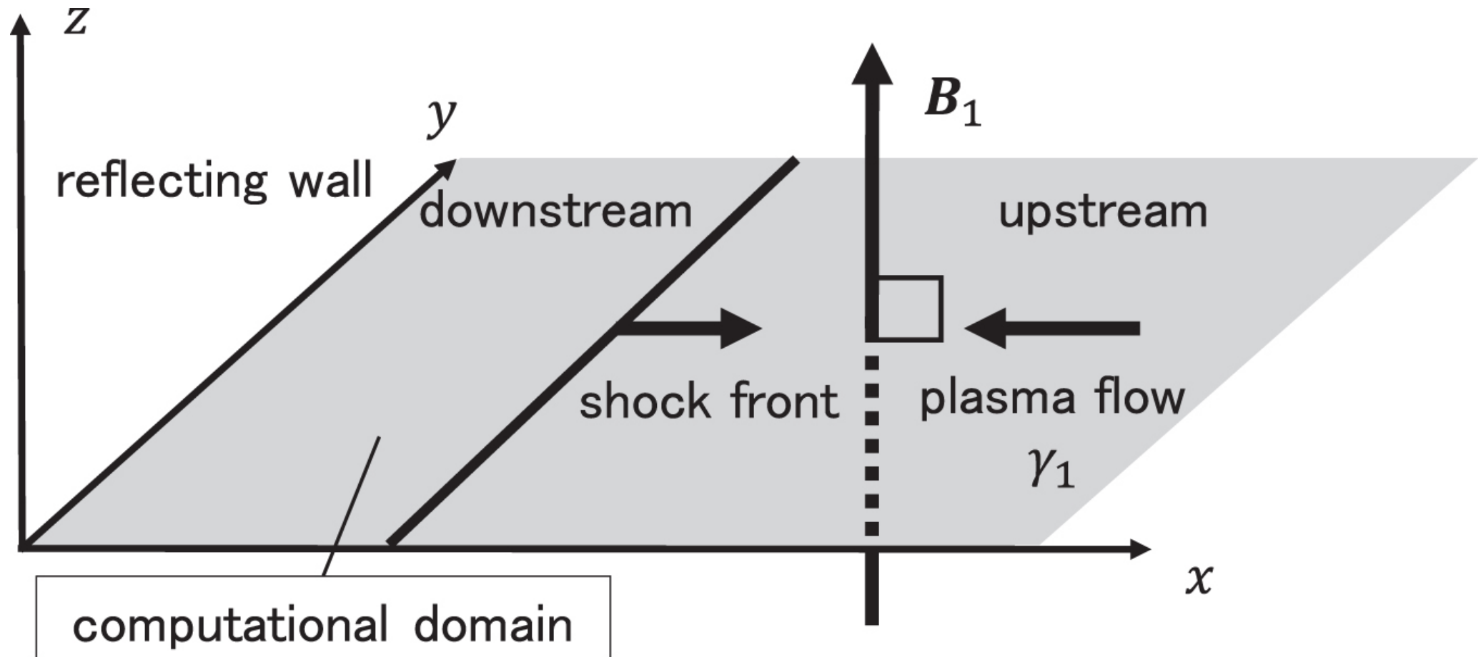
Figure 1. from Particle Acceleration by Pickup Process Upstream of Relativistic Shocks null 2022 APJ 924 108 doi:10.3847/1538-4357/ac38aa https://dx.doi.org/10.3847/1538-4357/ac38aa © 2022. The Author(s). Published by the American Astronomical Society.
