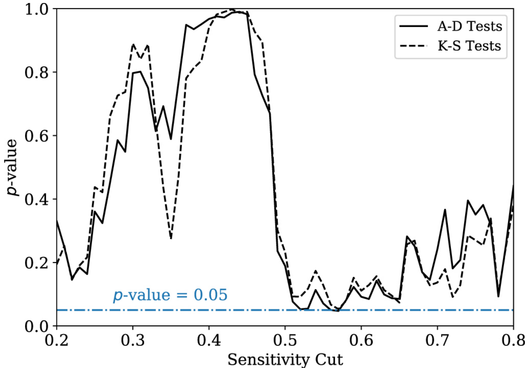
Figure 7. from No Evidence for Galactic Latitude Dependence of the Fast Radio Burst Sky Distribution null 2021 APJ 923 2 doi:10.3847/1538-4357/ac33ad https://dx.doi.org/10.3847/1538-4357/ac33ad © 2021. The Author(s). Published by the American Astronomical Society.
